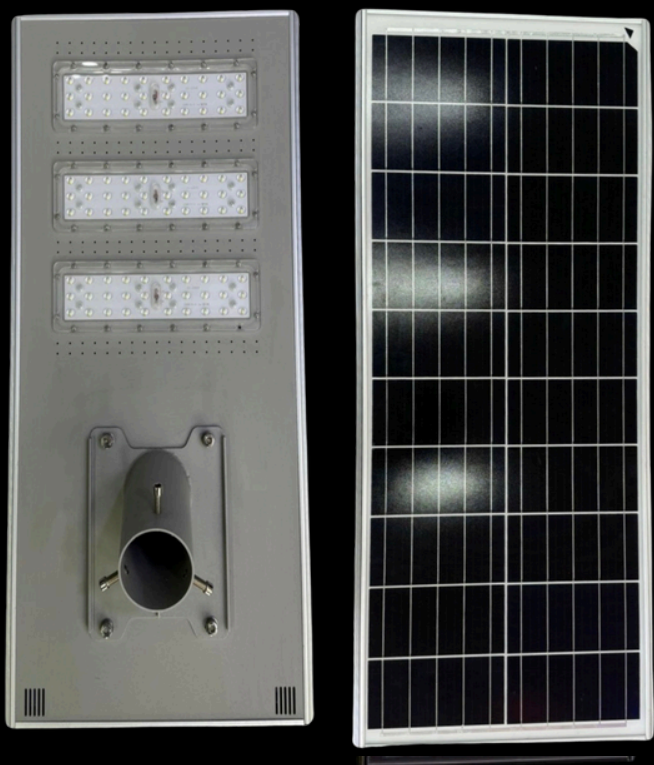
LAMPARA SOLAR ALL IN ONE IP66/ 300W MODELO: LA-10
