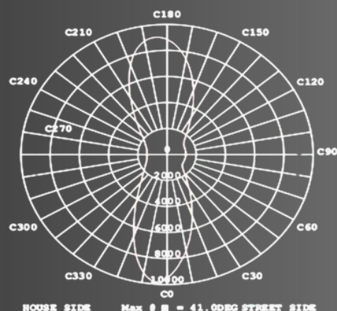
MAX INTENSITY CONE SURFACE DISTRIBUTION DIAGRAM
