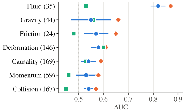
Attribution: this family vs. another violation
