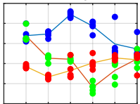
secretion system
