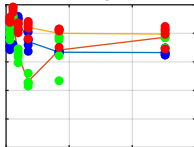
two-component
