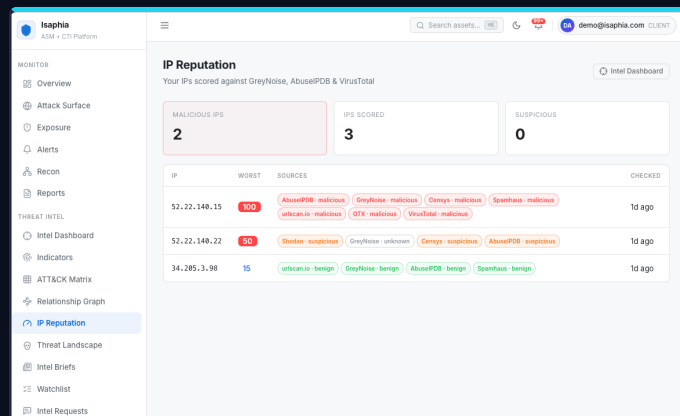
IP REPUTATION — MULTI-SOURCE CONSENSUS SCORING
