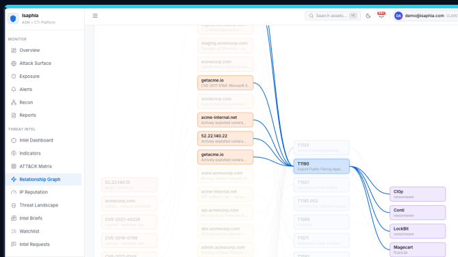
IOC RELATIONSHIP GRAPH — INDICATOR → FINDING → TECHNIQUE → ACTOR
