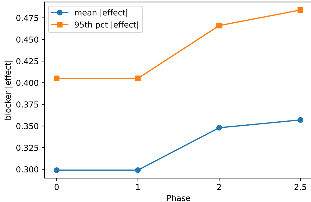
Blocker effect magnitude grows as attention is de-biased
