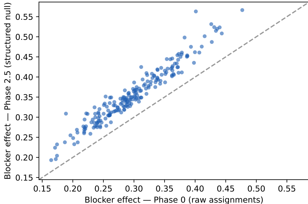
Blocker plus-minus: rank preserved (Spearman 0.97), magnitude sharpened by de-biasing
