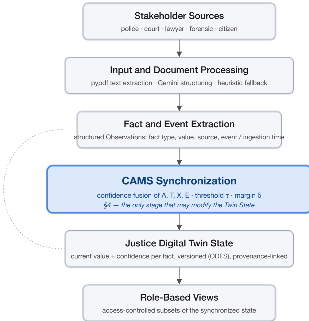
Fig. 1. NyayaOS Justice Digital Twin architecture. CAMS (highlighted) is the sole boundary between raw extracted observations and the synchronized case state.
