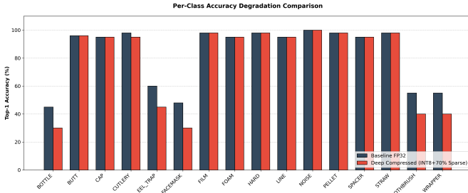
Fig. 4. Per-class Top-1 accuracy for the FP32 baseline (dark blue) and the Deep Compressed INT8 + 70% sparse model (red). Classes with sparse validation representation (BOTTLE, EEL_TRAP, FACEMASK, TOOTHBRUSH, WRAPPER) collapse under compression, identifying class imbalance as the primary constraint on per-class robustness.
