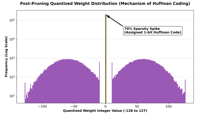
Fig. 1. Post-pruning quantized weight distribution (log scale) for the 70% sparse INT8 model. The zero-bin spike exceeds 10^4 frequency, two orders of magnitude above non-zero weight bins, and is assigned a 1-bit Huffman codeword, driving the 74.6% payload reduction from 5.98 MB to 1.52 MB.
