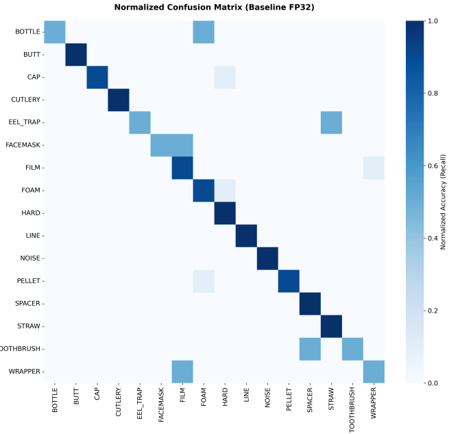
Fig. 2. Normalized confusion matrix for the FP32 baseline across all 16 morphological classes. The strong diagonal confirms per-class discriminability. Off-diagonal confusions primarily occur between FACEMASK/FILM and STRAW/EEL_TRAP, reflecting shared elongated and irregular edge morphology respectively.
