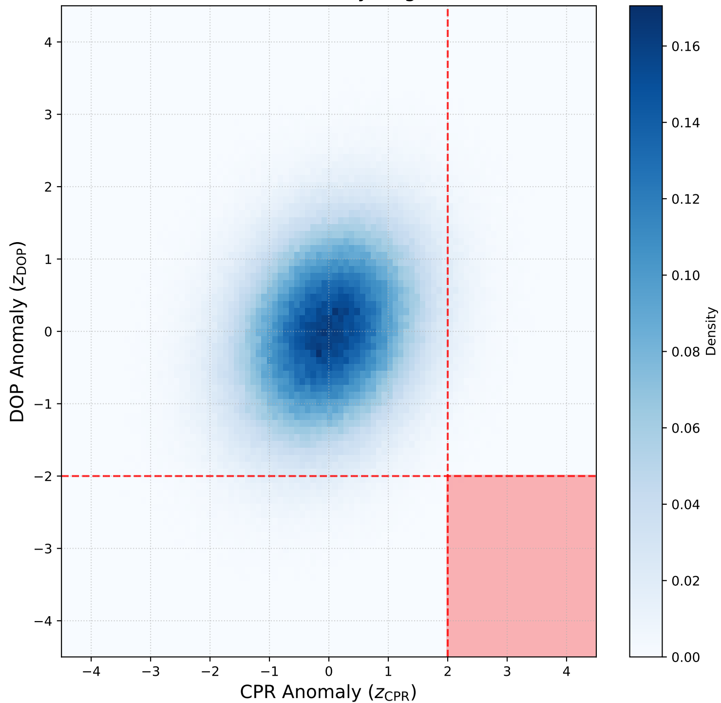
Bivariate Distribution of Dry Regolith ( r = 0.225 )
