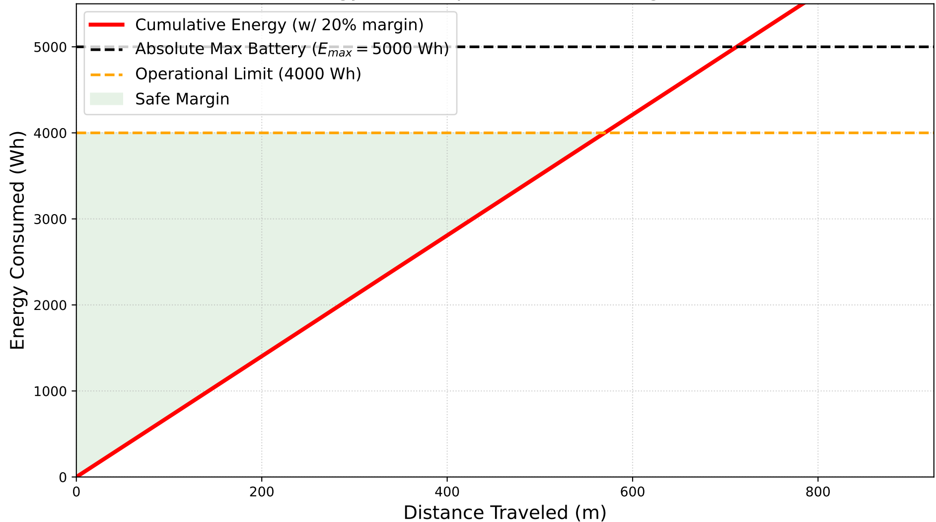
Rover Energy Consumption Profile During A* Traverse
