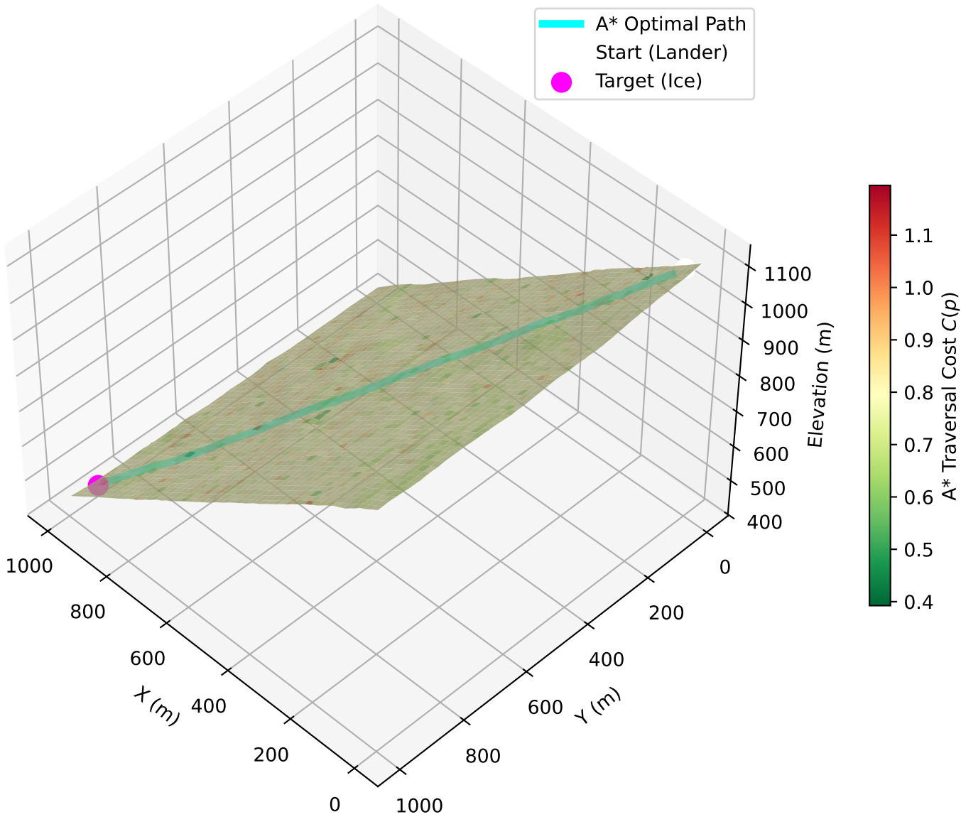
3D Rover Traverse on LOLA DEM (Colored by Risk/Slope Cost)
