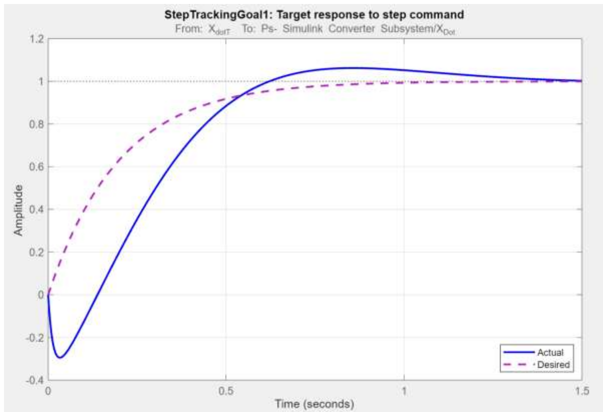
Figure 15 Target response with manual gains
