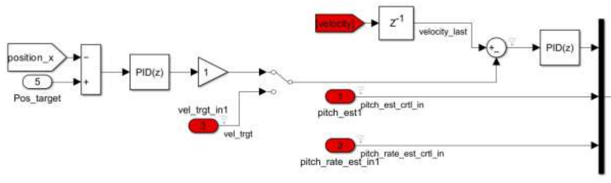
Figure 55 The cascaded PID controller implementation for challenge 3
