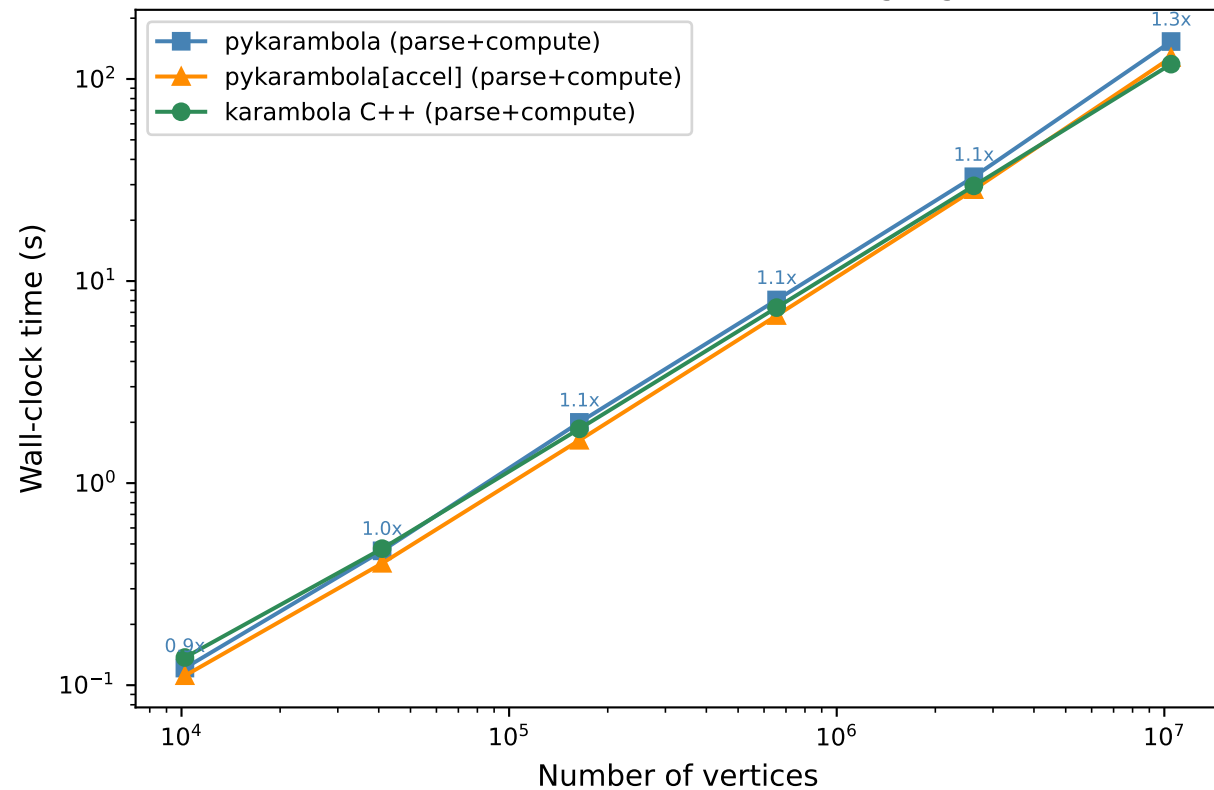
Number of vertices vs Time (log-log)
