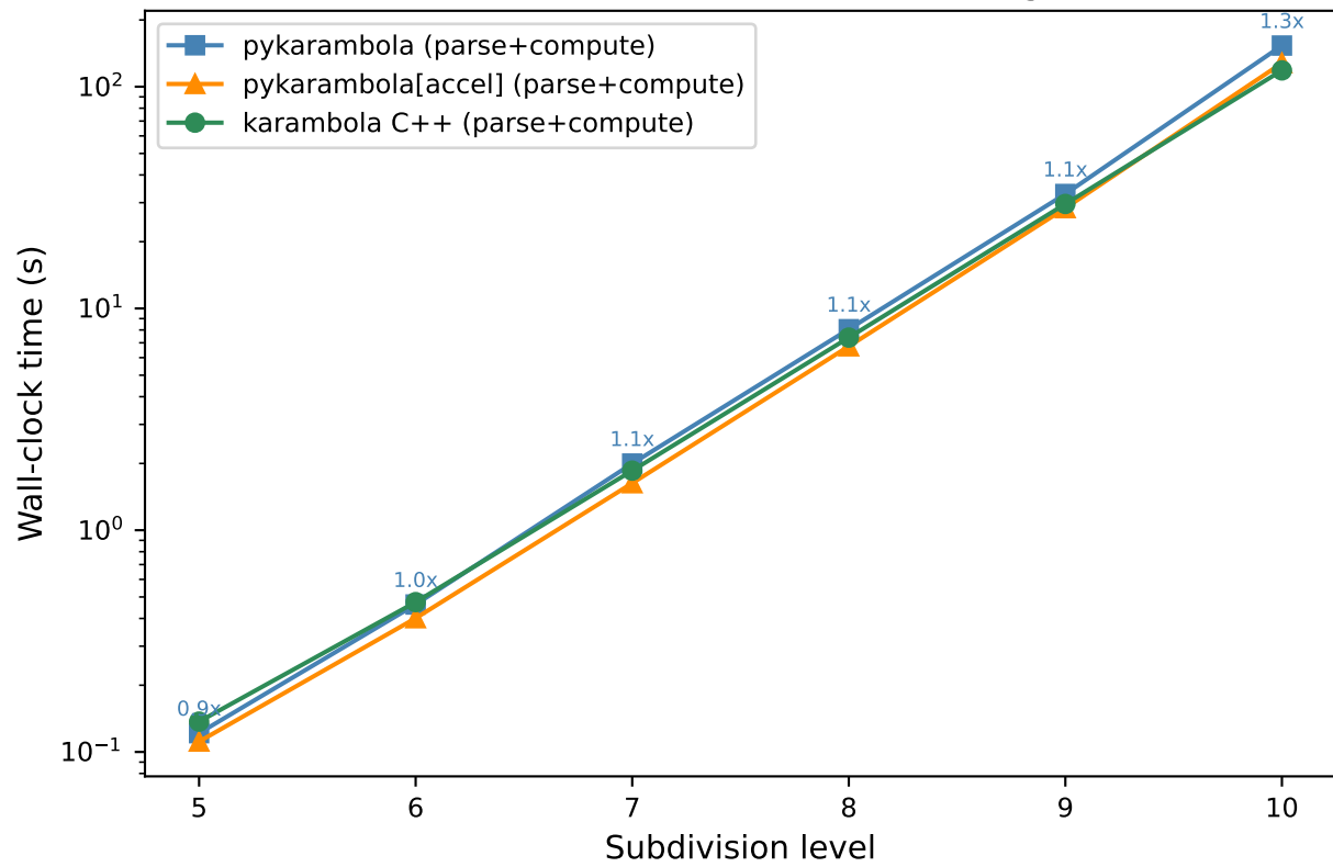
Subdivision level vs Time (semi-log)
