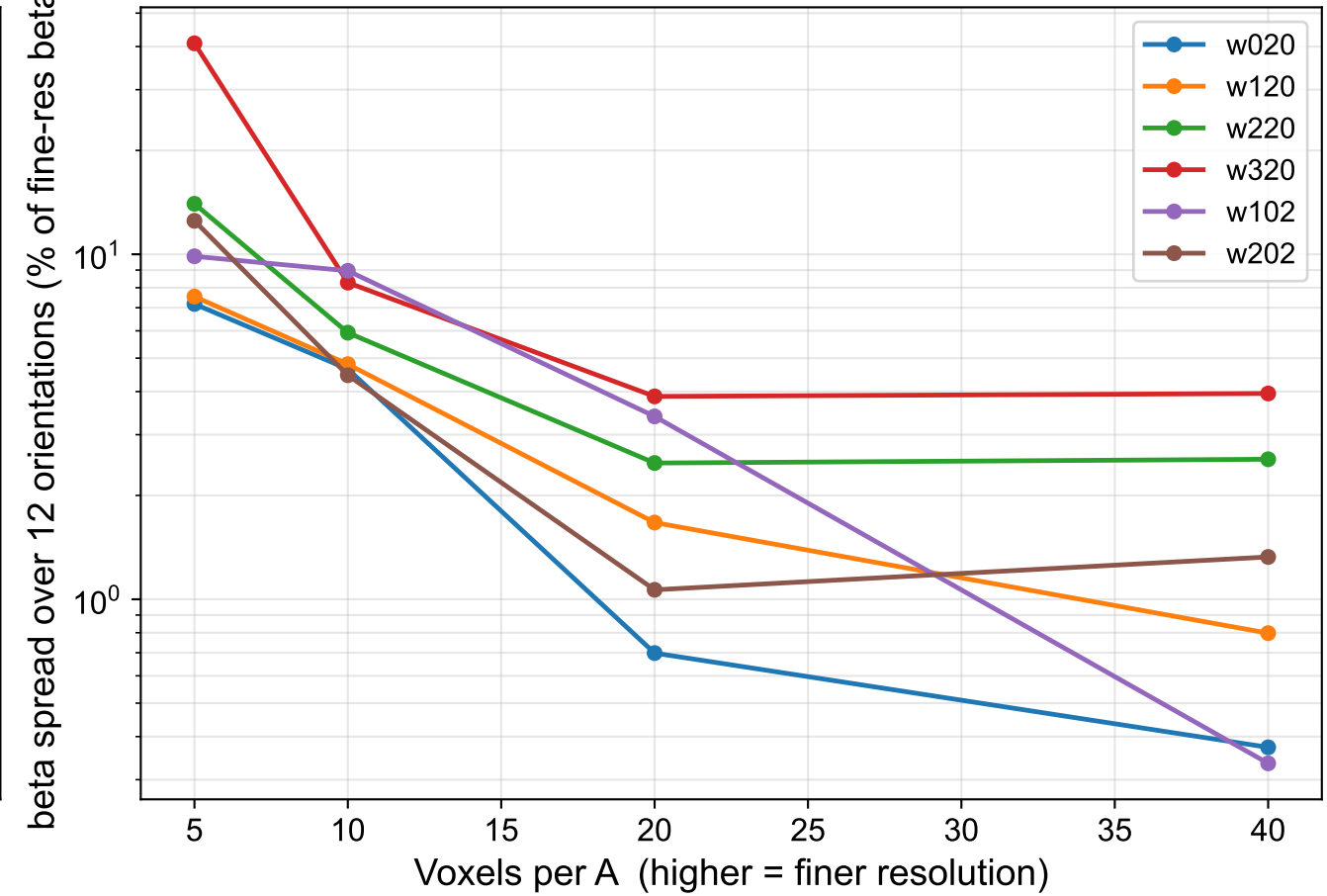
(b) Rank-2 tensors — orientation-dependent beta spread
