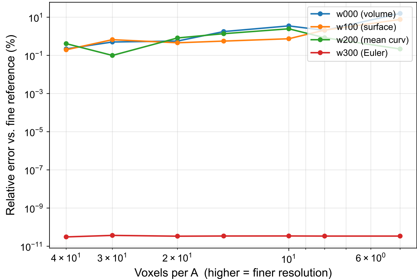
(a) Scalars — asymptotic convergence (no orientation bias)
