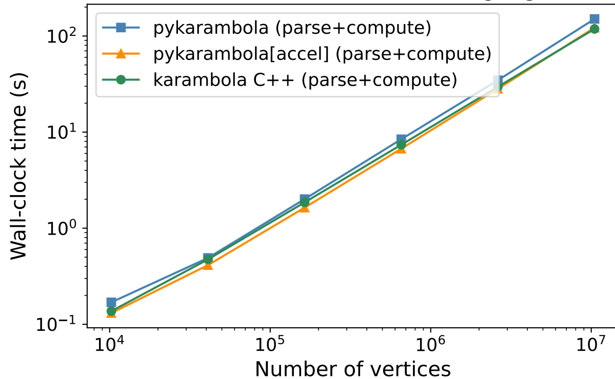
Runtime versus mesh size (log-log)
