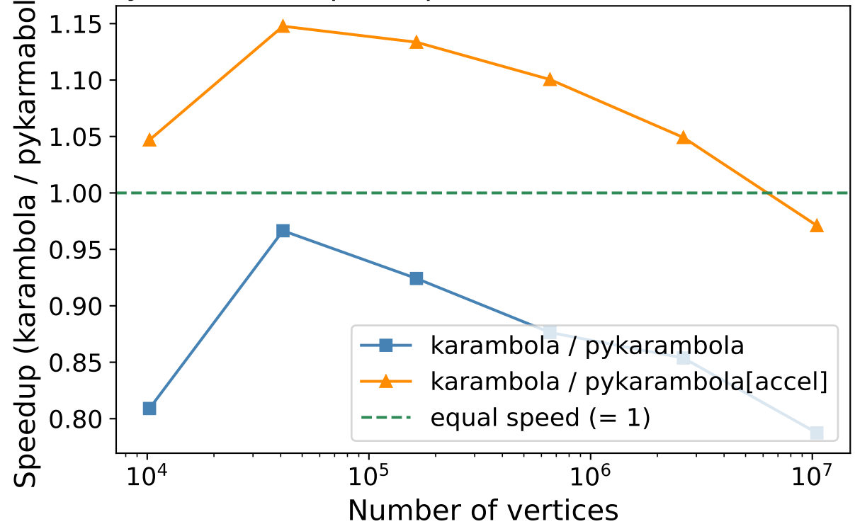
Pykarmabola speedup relative to C++ karmabola
