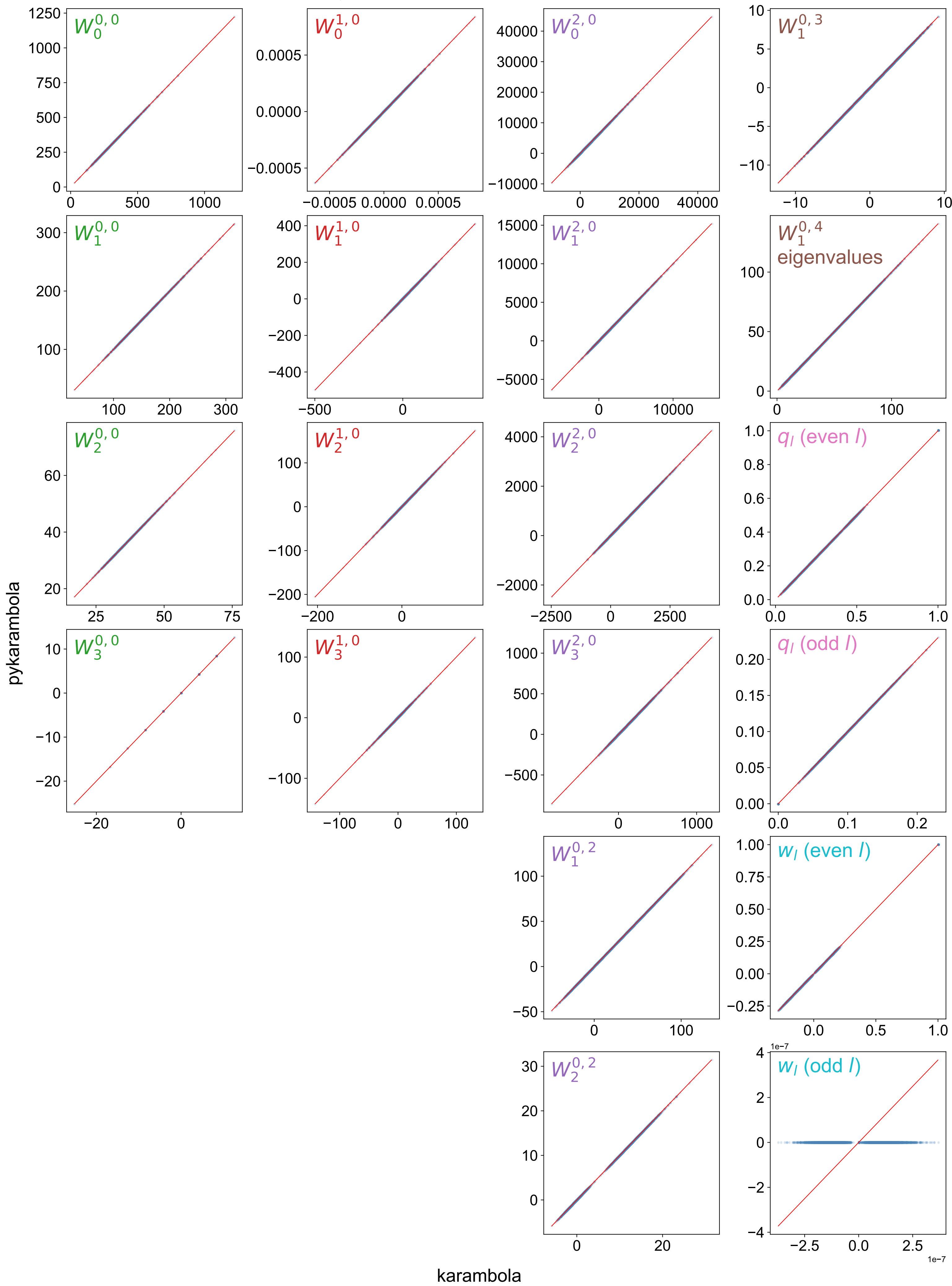
Validation: pykarambola vs C++ karambola — 28^3 voxels
