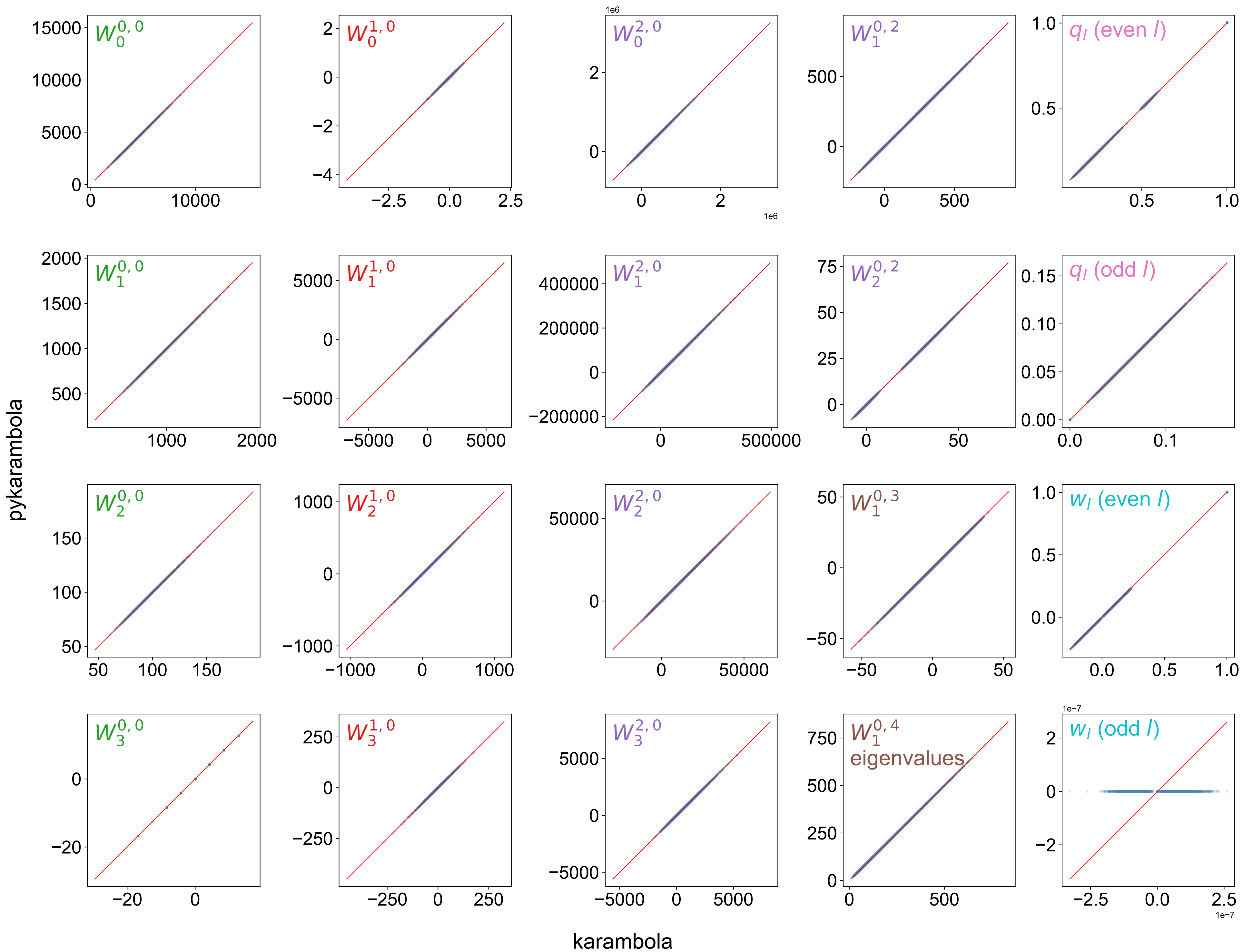
Validation: pykarambola vs C++ karambola — 64^3 voxels
