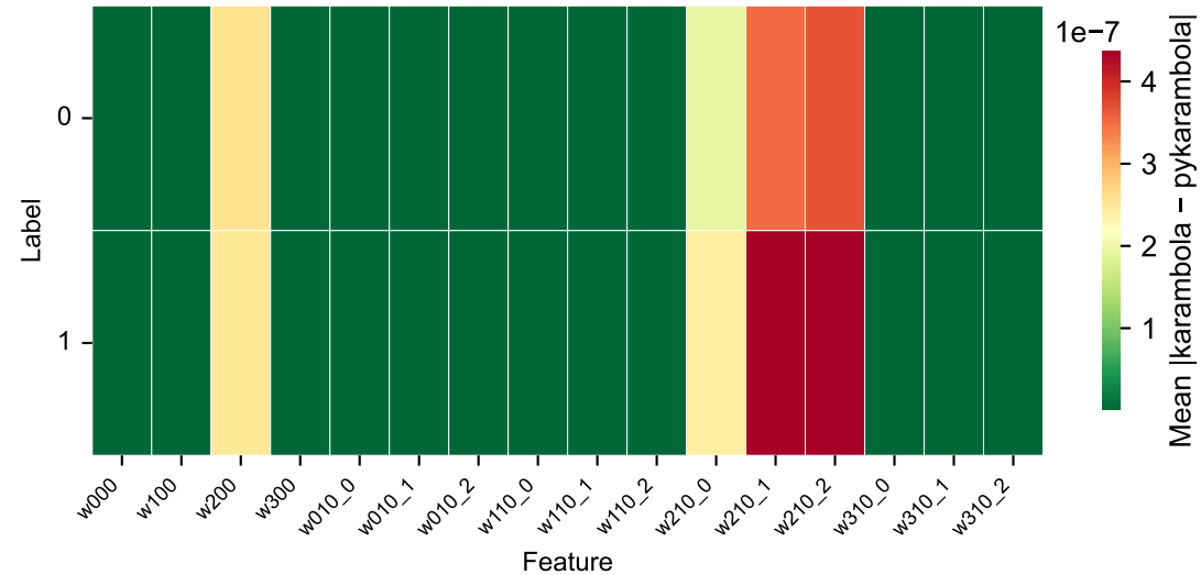
adrenal3d 28 3
