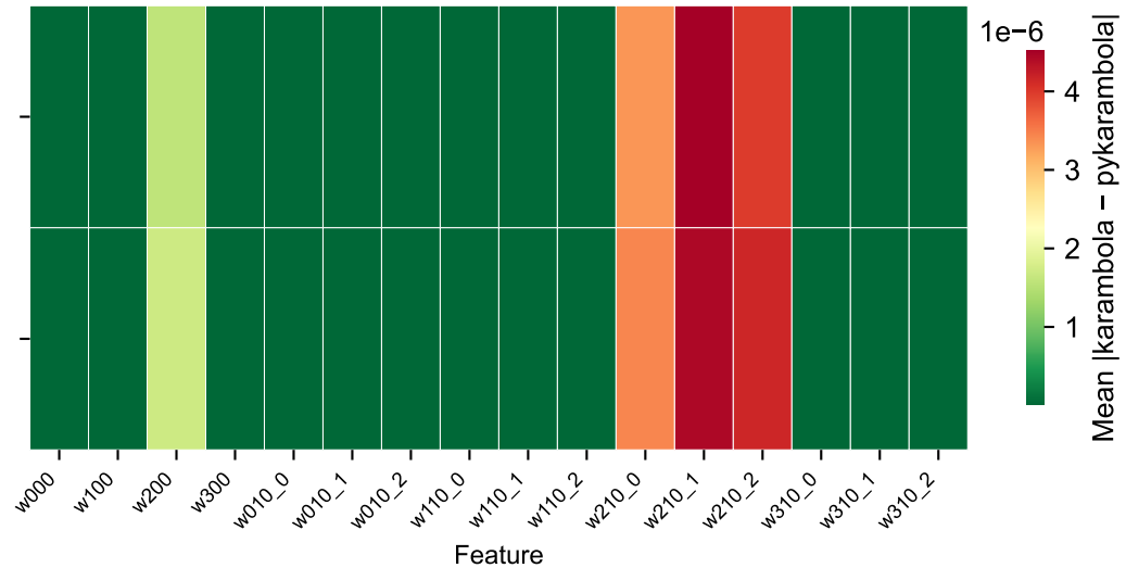
adrenal3d 64 3
