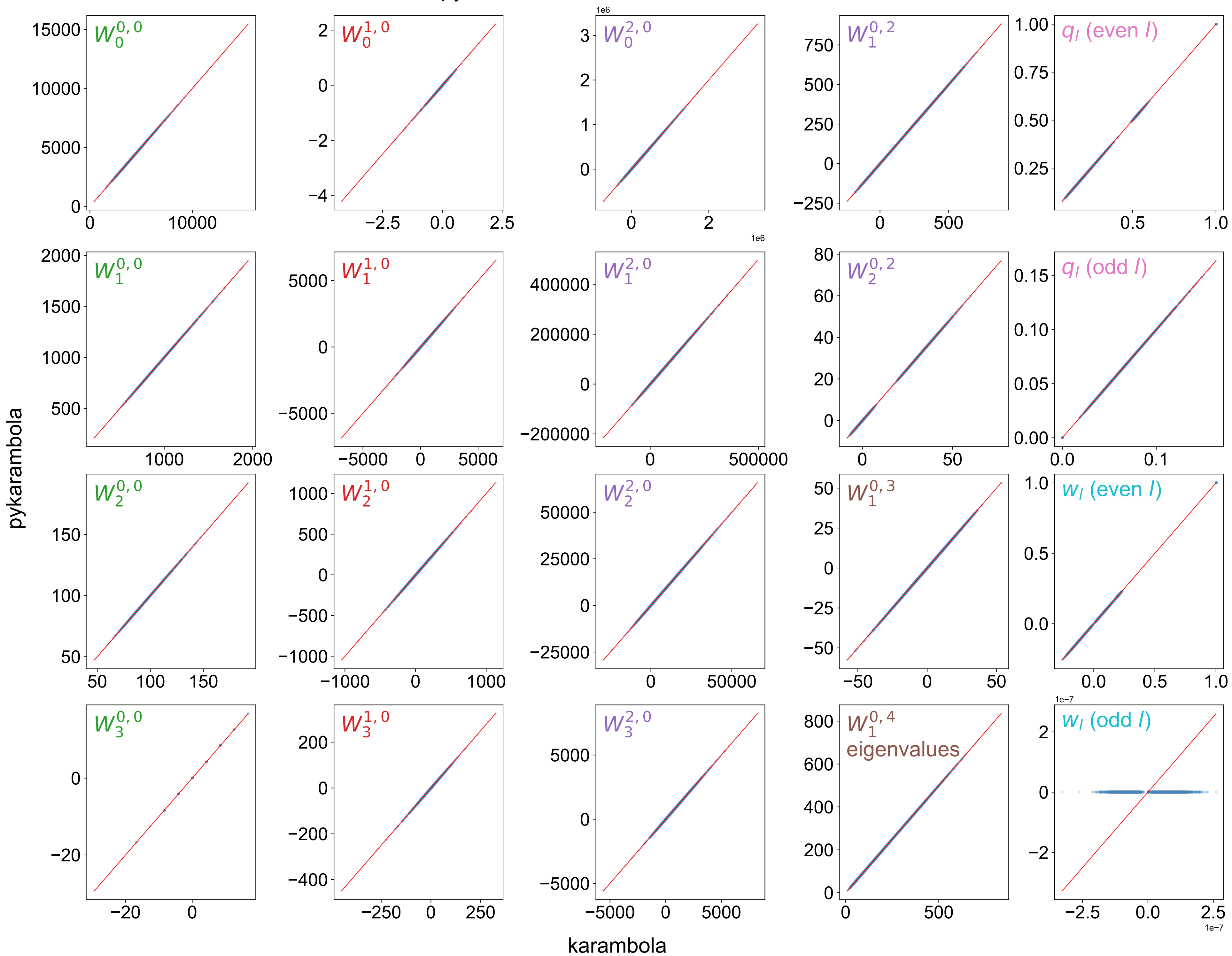
Validation: pykarambola vs C++ karambola — 64^3 voxels
