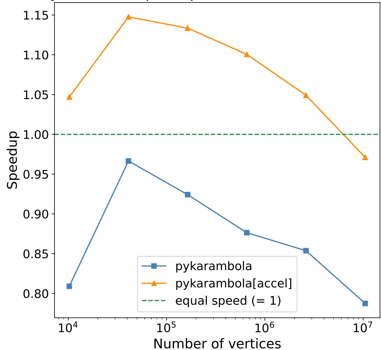
Pykarmabola speedup relative to C++ karmabola
