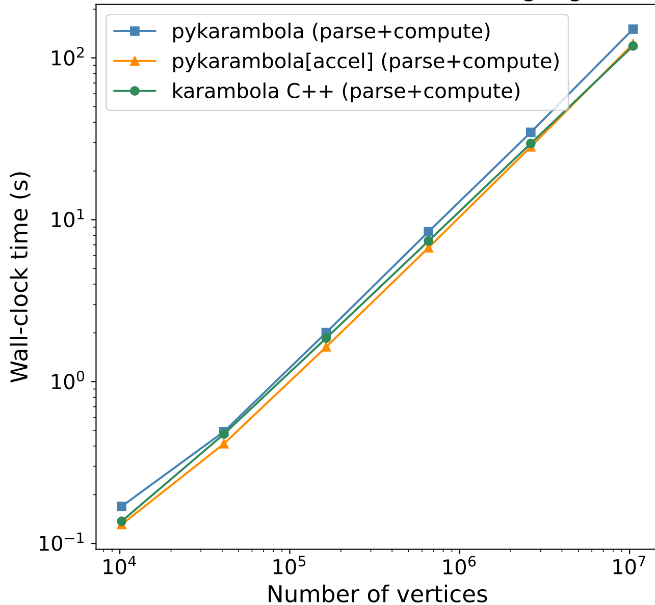
Runtime versus mesh size (log-log)
