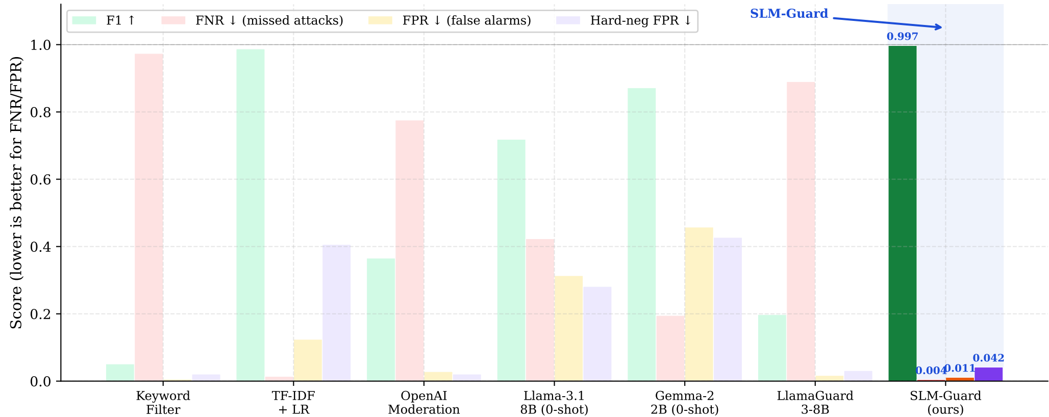
Guardrail Comparison on SE Attack Test Set (↑ higher F1 better ↓ lower FNR/FPR better)
