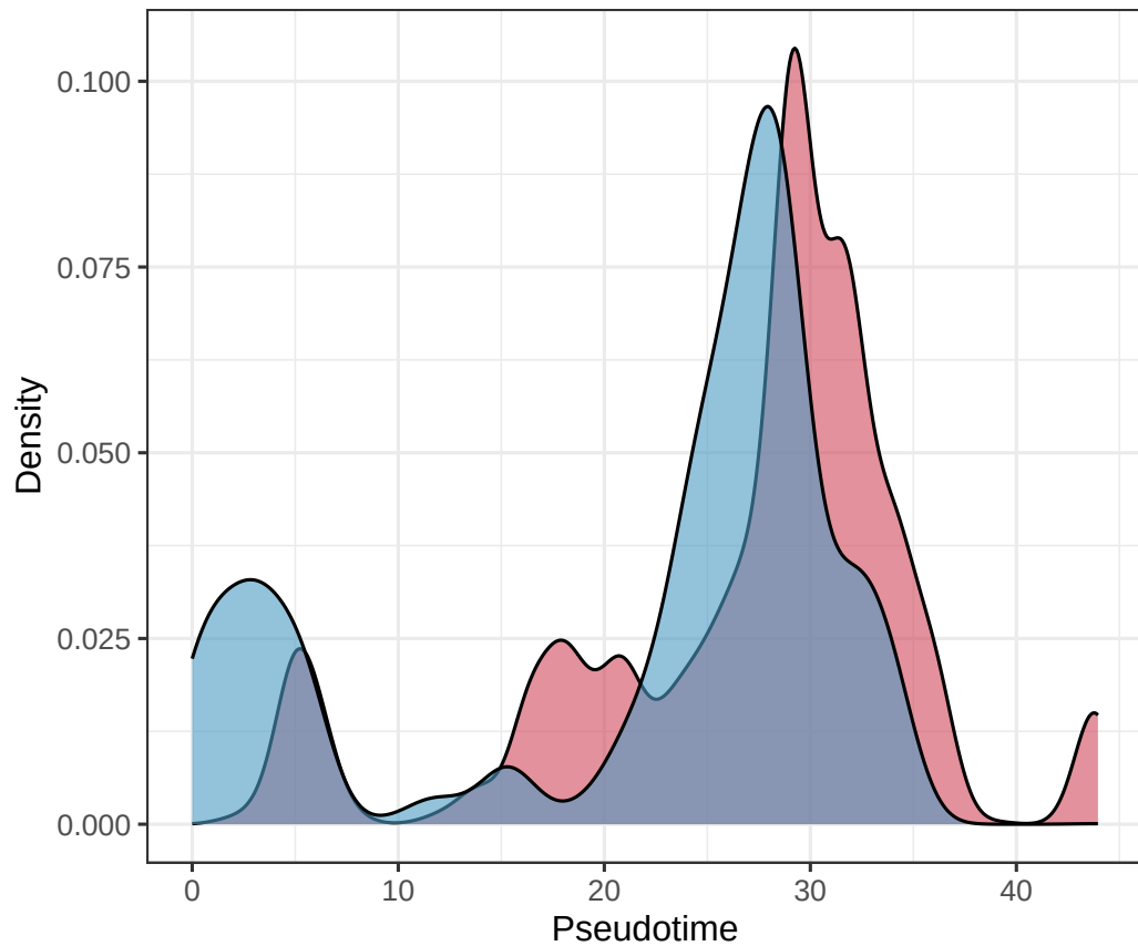
Pseudotime density: AD vs Control — OligoLineage
