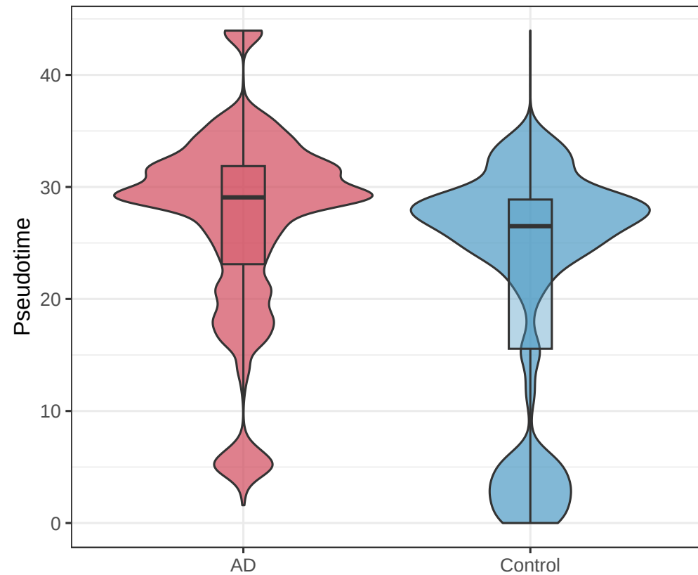
Pseudotime by condition — OligoLineage
