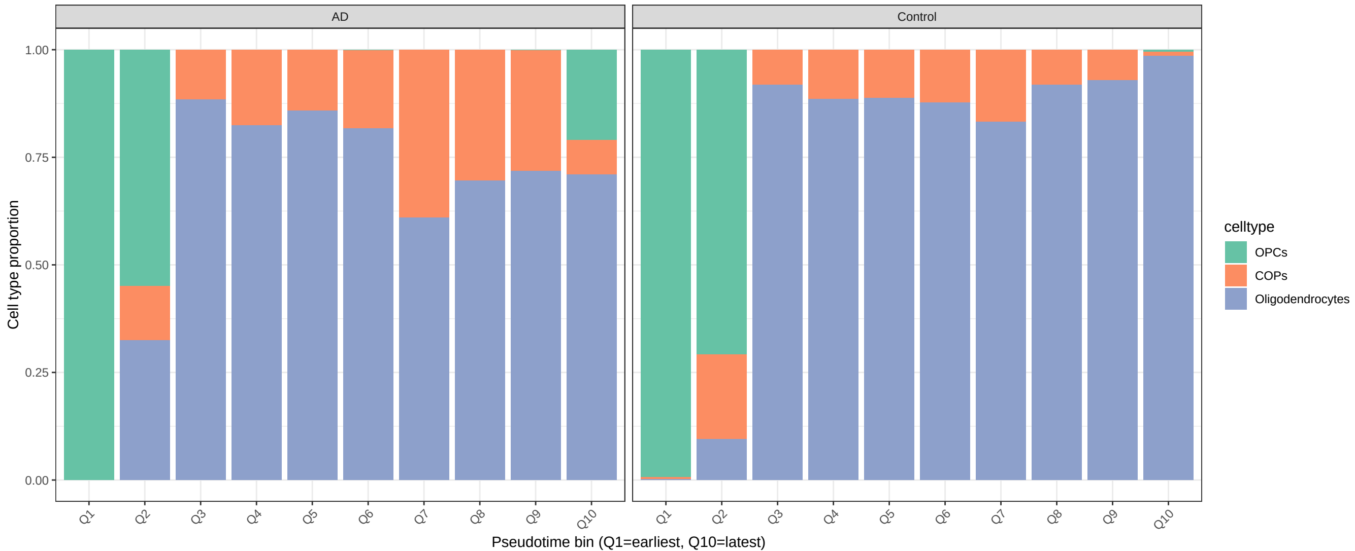
Cell-type composition along pseudotime — OligoLineage
