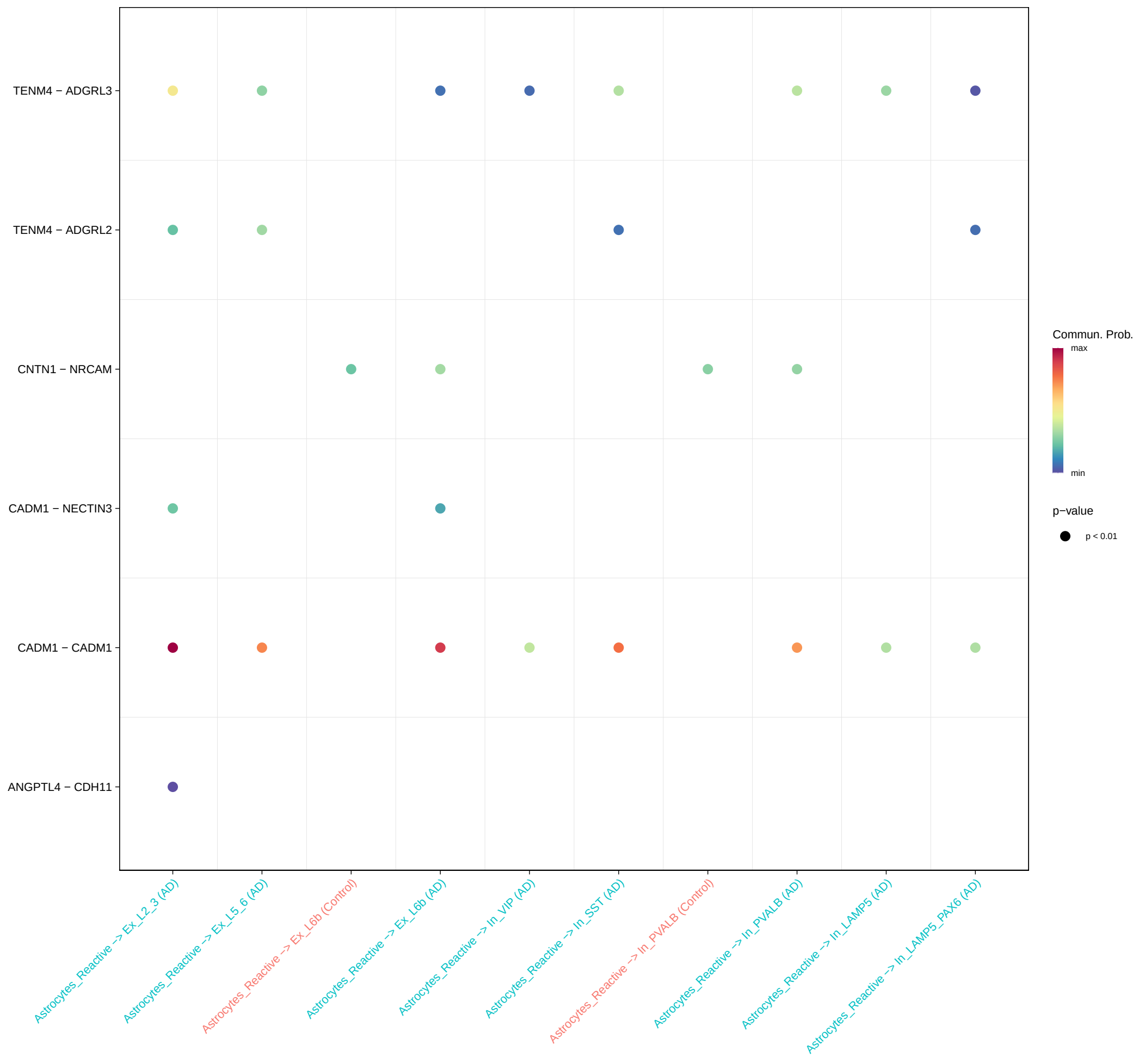
Up in AD — ReactiveAstro_to_Neurons
