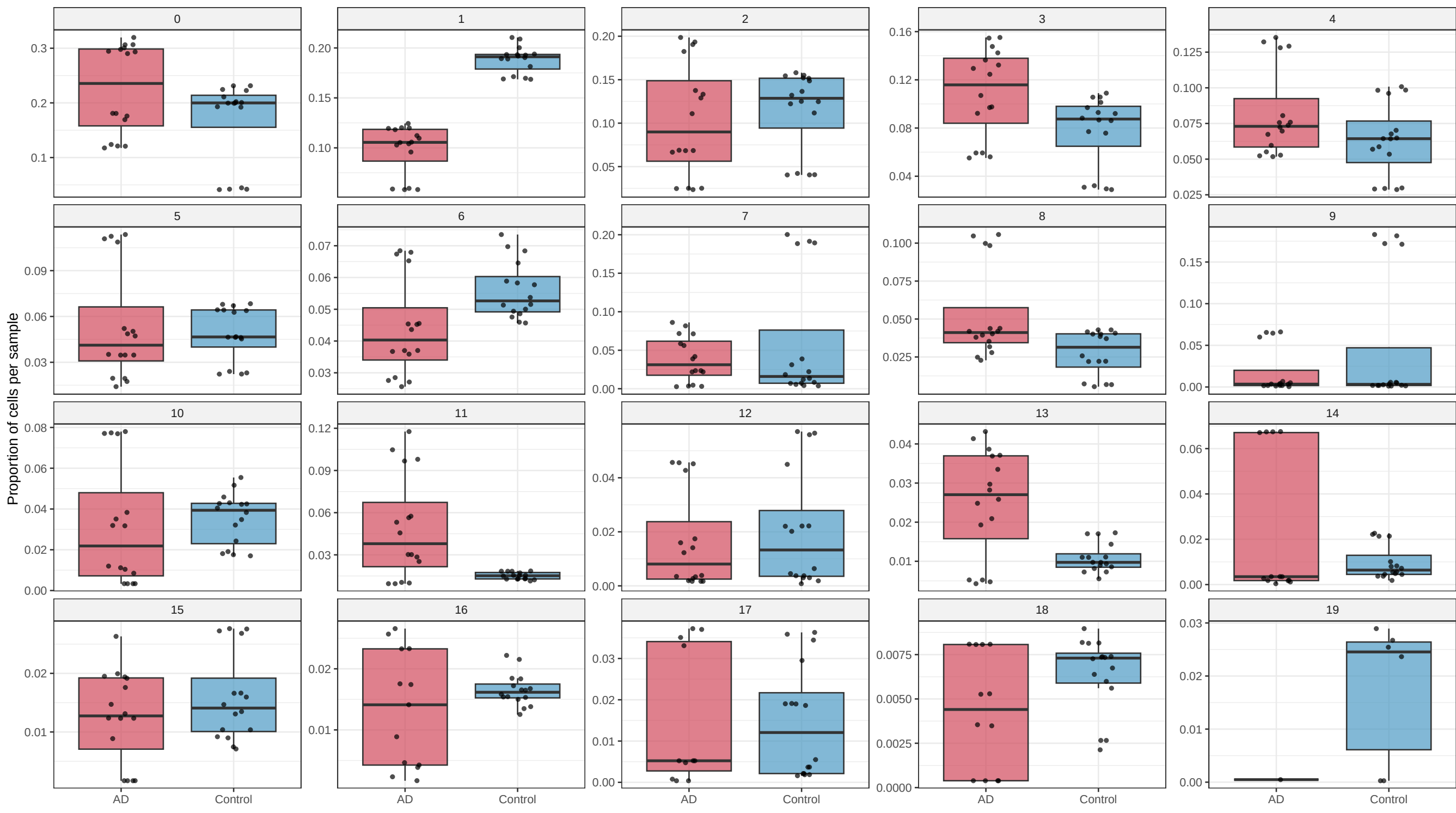
C. Per-cluster proportions: AD vs Control (each dot = sample)
