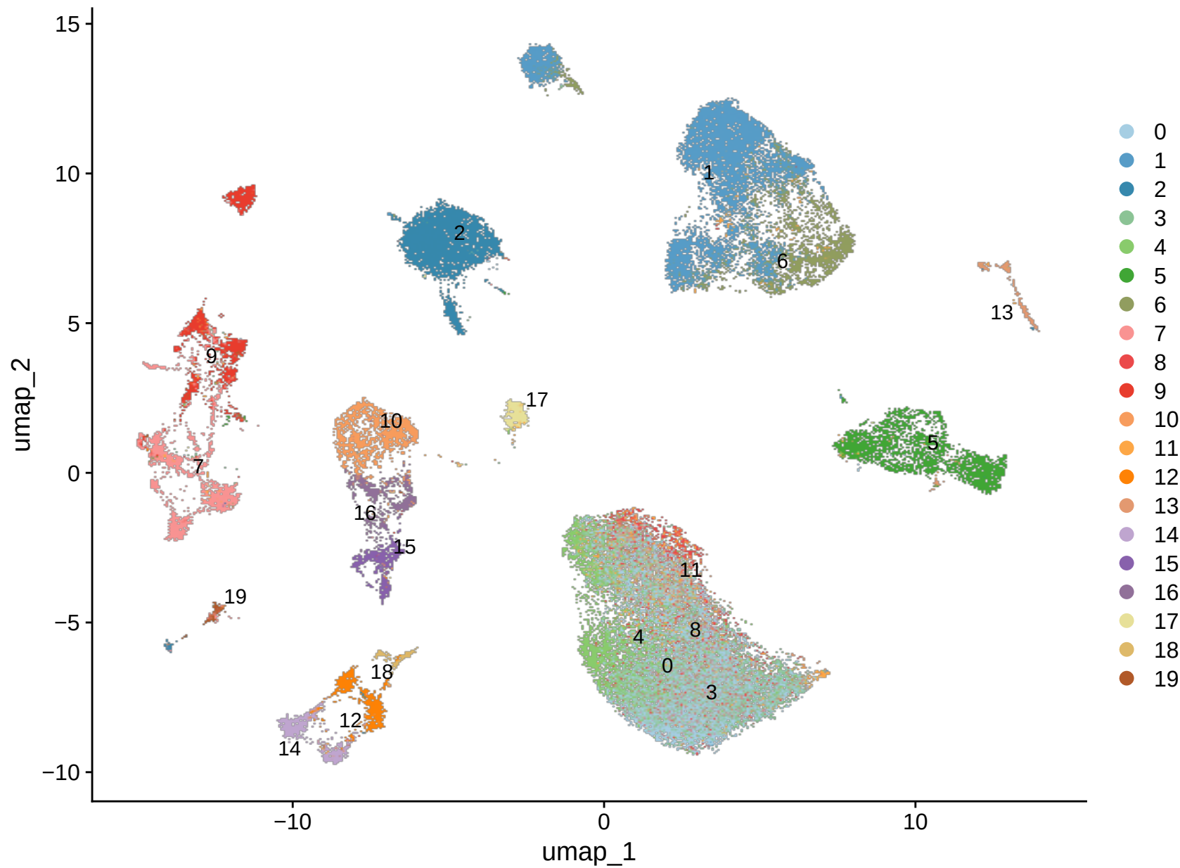
UMAP — 20 clusters at res 0.5 (mt-removed)
