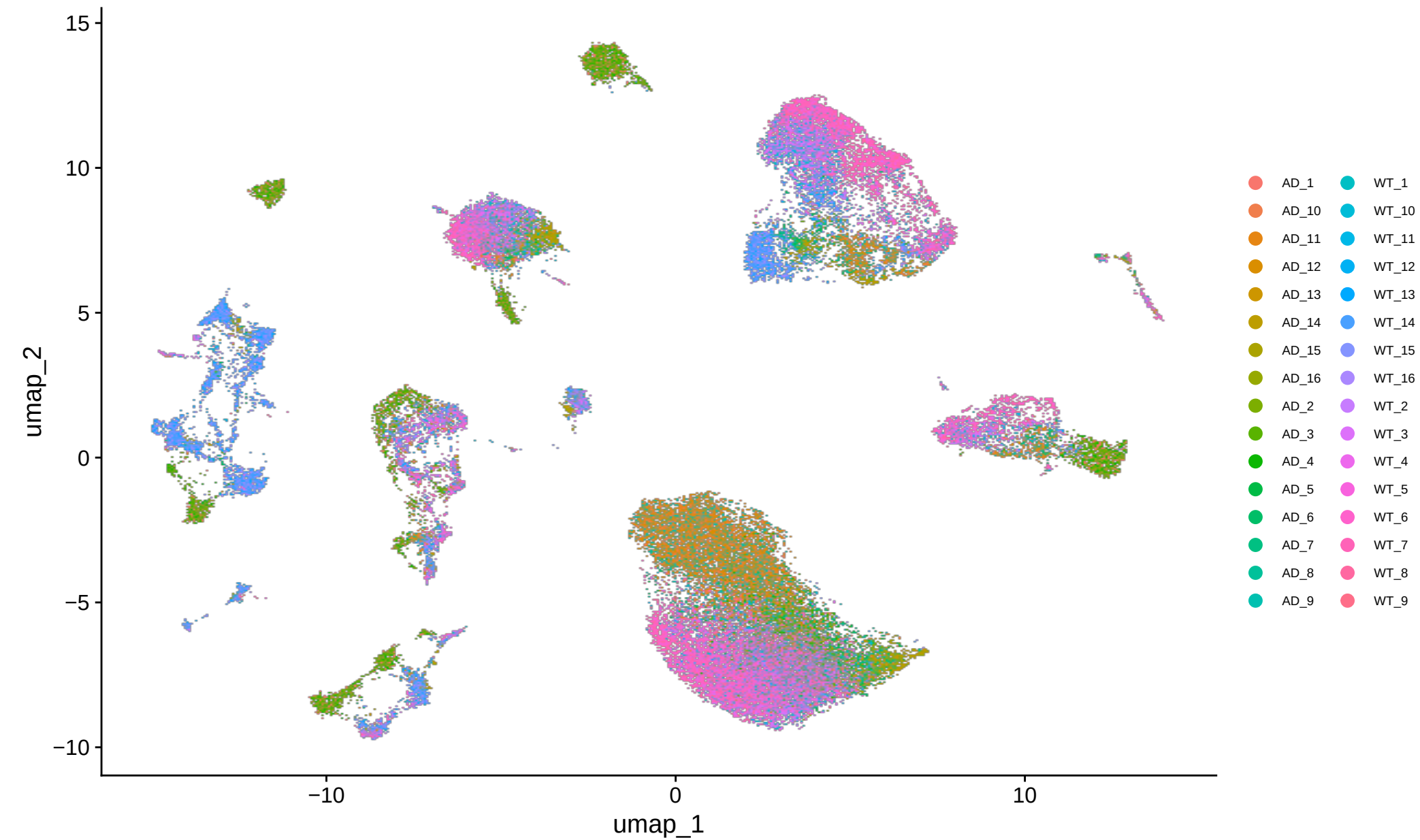
UMAP — by sample (integration check)
