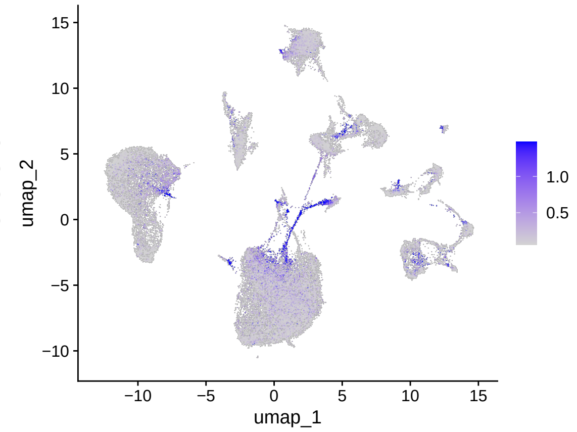
percent.mt
