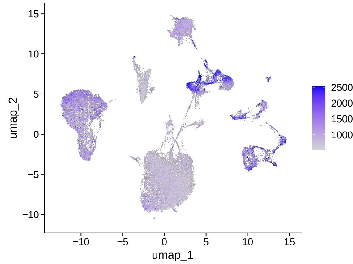
nCount_RNA
