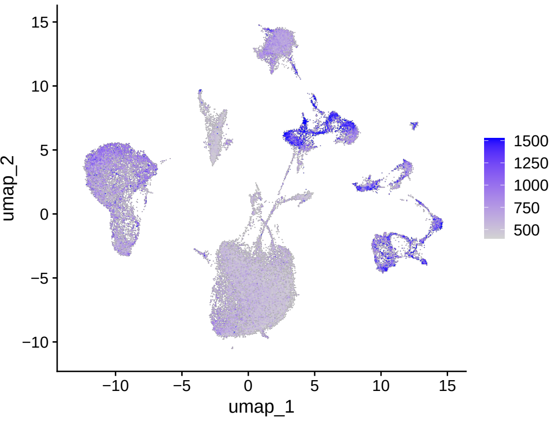
nFeature_RNA
