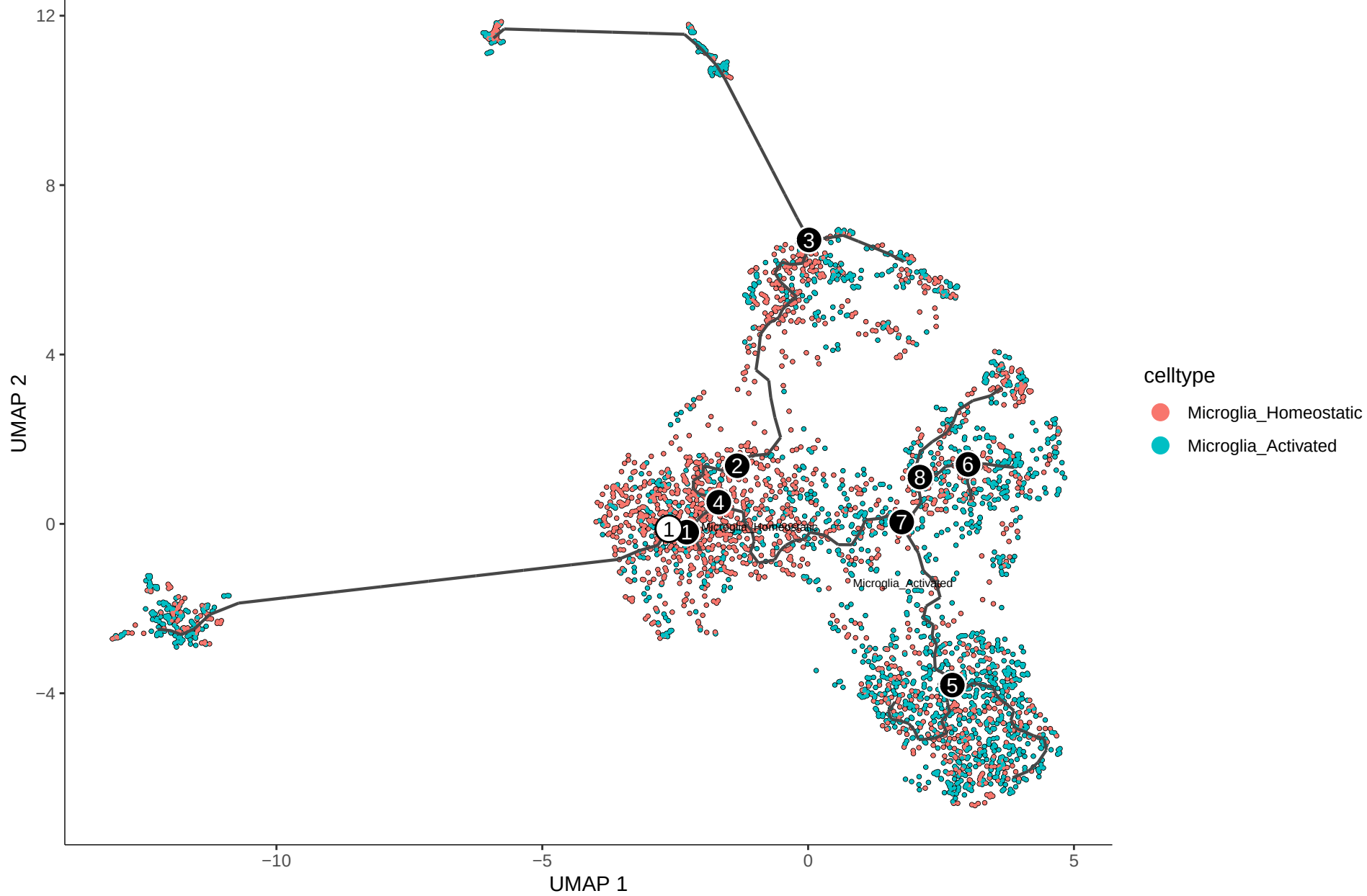
MicrogliaActivation — cell types
