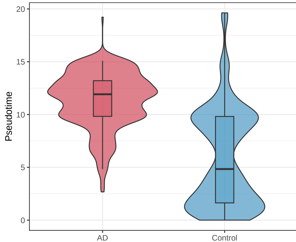
Pseudotime by condition — MicrogliaActivation
