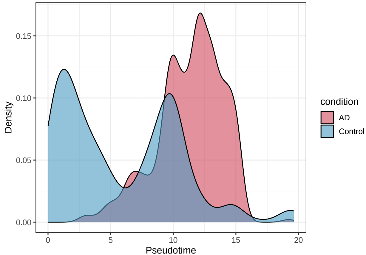
Pseudotime density: AD vs Control — MicrogliaActivation
