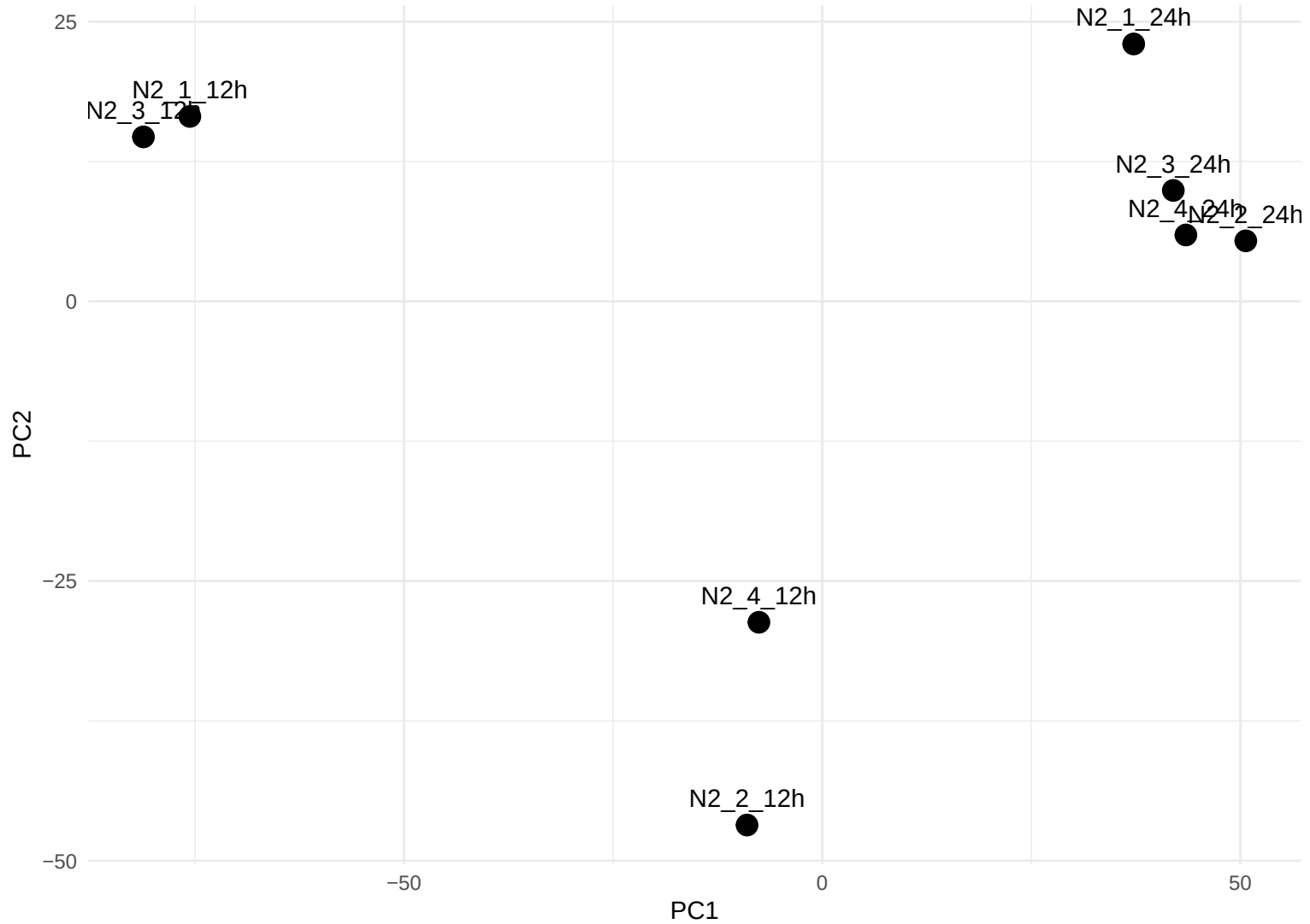
PCA of RNA-seq Samples
