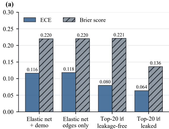
Calibration metric
