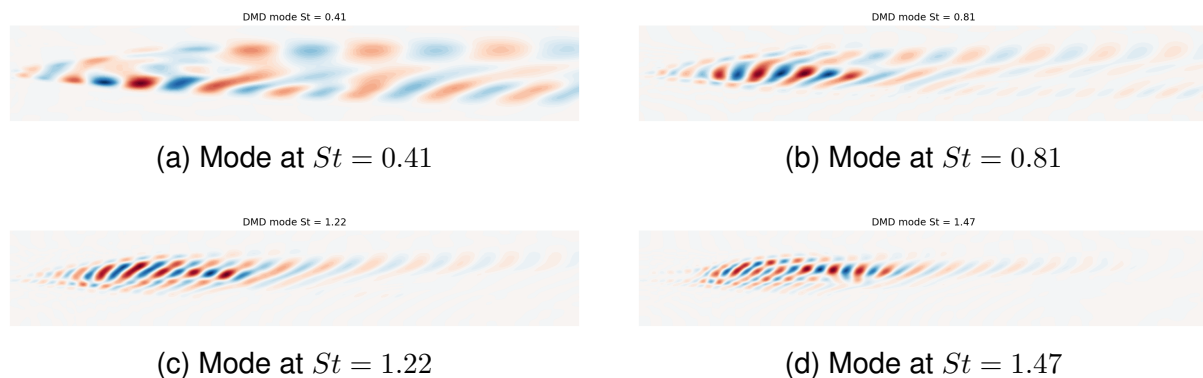
Figure 6: DMD temperature modes for the 1500 K dataset at the main harmonic frequencies ( St = 0.41, 0.81, 1.22, 1.47 ), corresponding to f, 2f, 3f , and 4f respectively.
