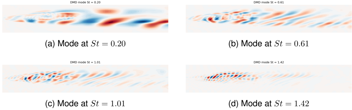
Figure 7: DMD temperature modes for the 1500 K dataset at the quasi-periodic combination frequencies ( St = 0.20, 0.61, 1.01, 1.42 ), highlighted by green ellipses in Figure 5.
