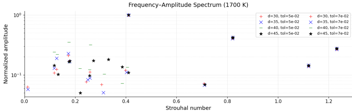
Figure 6: Normalised DMD mode amplitudes as a function of Strouhal number for the 1700 K dataset, for d \in \{35, 40, 45\} and \varepsilon_{\text{tol}} \in \{5 \times 10^{-2}, 7 \times 10^{-2}\} .
