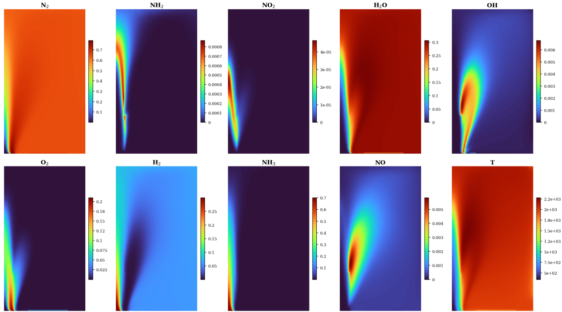
Figure 10: Thermochemical variables of the ( \phi = 1.2 , H_2 = 0.3 vol%, p = 2 atm) operating conditions point in the ULB-modified SPRF furnace.
