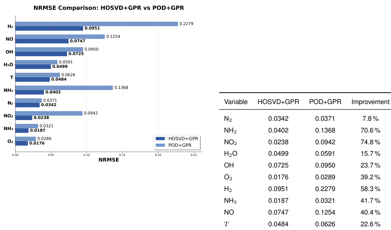
Figure 12: NRMSE comparison between HOSVD+GPR and POD+GPR across all predicted variables. The bar chart (left) and table (right) both show that HOSVD+GPR consistently outperforms POD+GPR, with the largest improvements observed for NH 2 (70.6 %), NO 2 (74.8 %), and H 2 (58.3 %).
