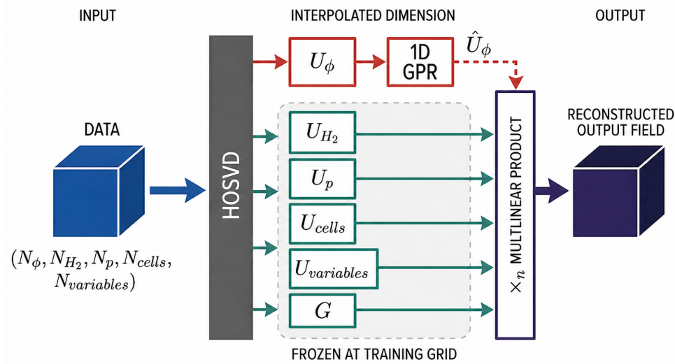
Figure 11: Schematic of the HOSVD+GPR pipeline.
