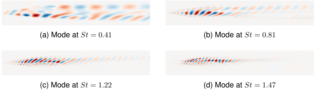
Figure 12: DMD temperature modes for the 1500 K dataset at the main harmonic frequencies ( St = 0.41, 0.81, 1.22, 1.47 ), corresponding to f, 2f, 3f , and 4f respectively.
