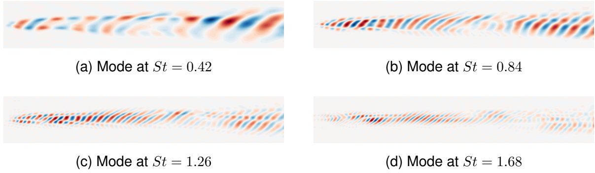
Figure 10: DMD temperature modes for the 1200 K dataset at the main harmonic frequencies ( St = 0.42, 0.84, 1.26, 1.68 ), corresponding to f, 2f, 3f , and 4f respectively.
