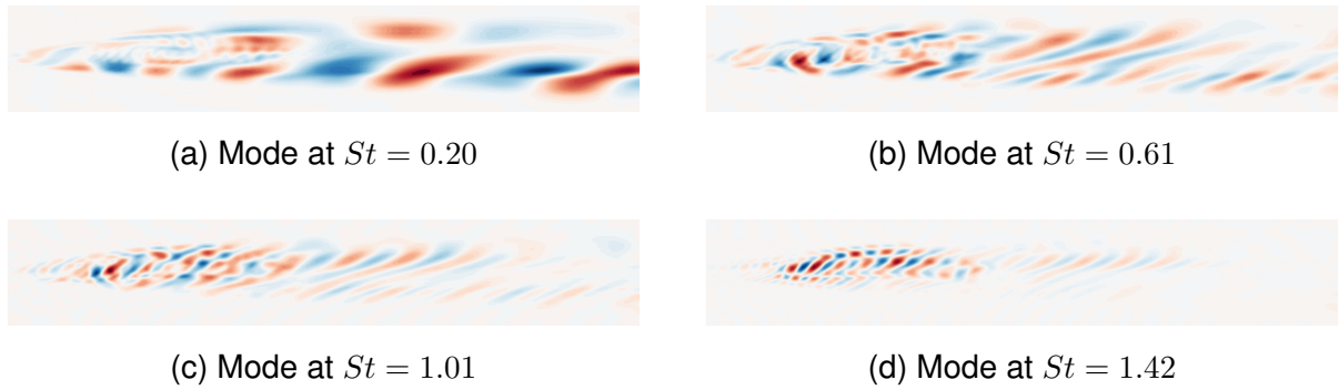
Figure 13: DMD temperature modes for the 1500 K dataset at the quasi-periodic combination frequencies ( St = 0.20, 0.61, 1.01, 1.42 ), highlighted by green ellipses in Figure 11.
