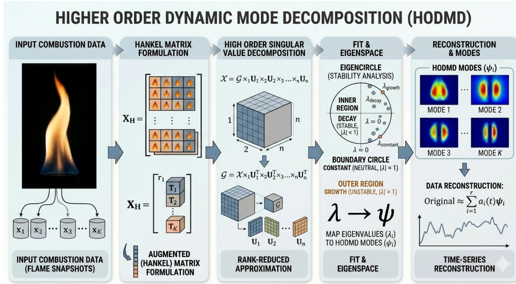
Figure 8: Scheme representing High Order Dynamic Mode Decomposition on combustion data
