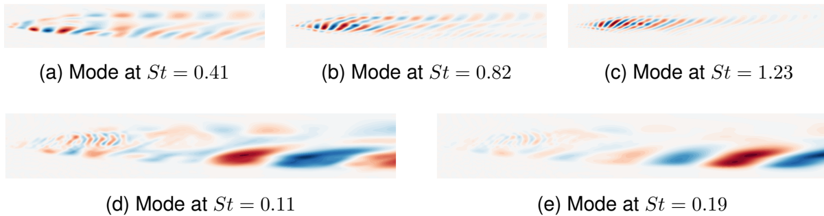
Figure 15: DMD temperature modes for the 1700 K dataset. Top row: modes at the three main harmonic frequencies ( St = 0.41, 0.82, 1.23 ). Bottom row: modes at the additional frequencies highlighted in blue in Figure 14 ( St = 0.11, 0.19 ).
