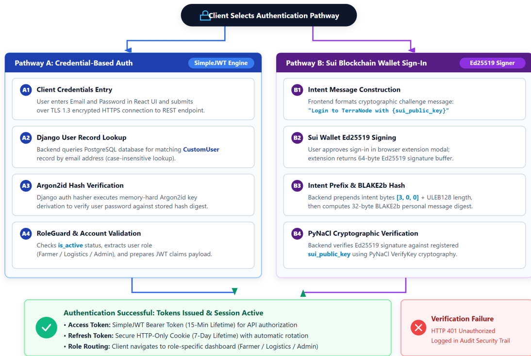
Figure 3.7: Authentication Flow Diagram
