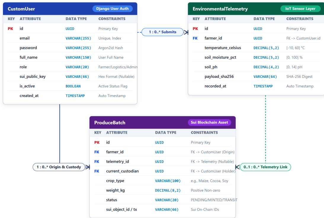
Figure 3.4: Entity-Relationship Diagram
