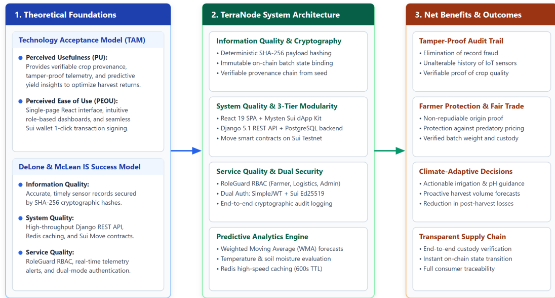
Figure 2.1: Conceptual Framework of the TerraNode System
