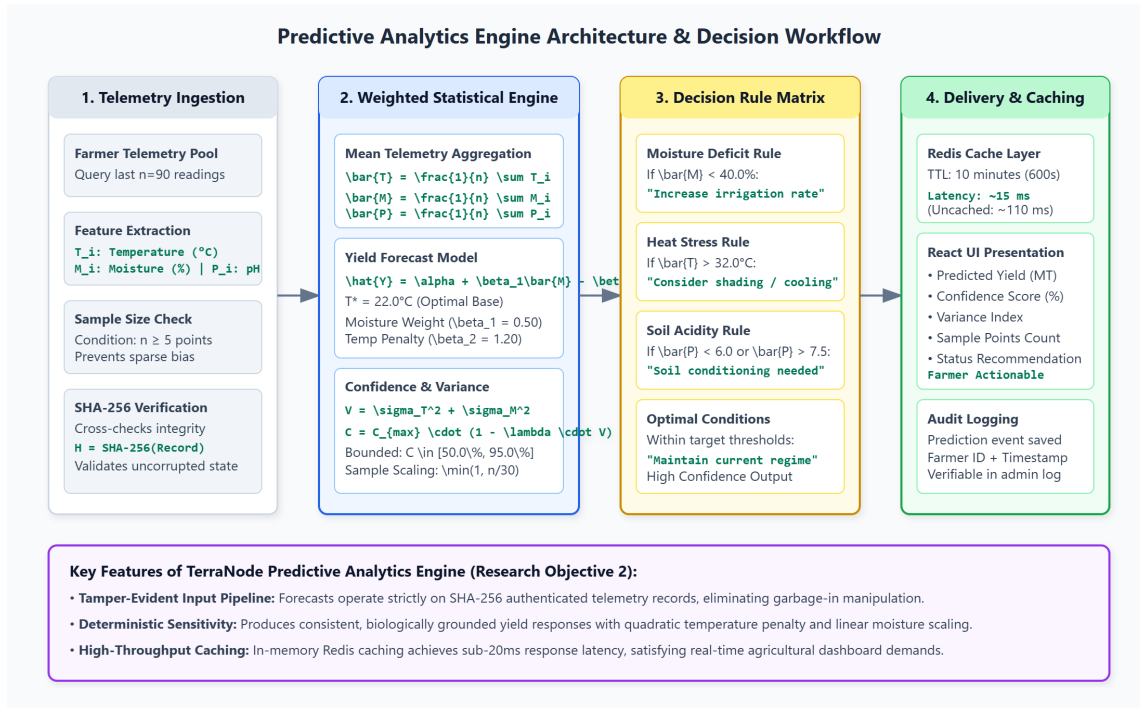
Figure 4.4: Predictive Analytics Engine Architecture and Decision Workflow
