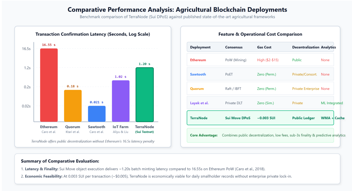
Figure 4.7: Comparative Performance Analysis of Agricultural Blockchain Deployments
