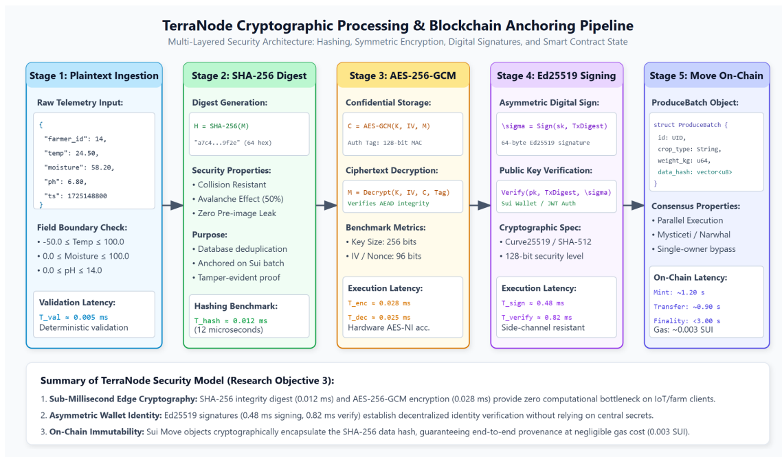
Figure 4.6: TerraNode Cryptographic Processing and Blockchain Anchoring Pipeline
