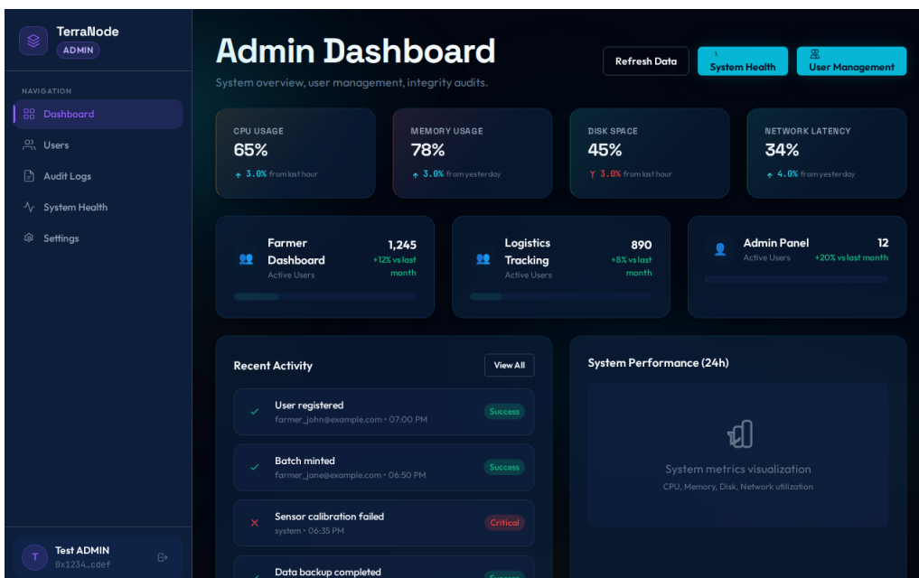
Figure 4.10: Administrator Dashboard
