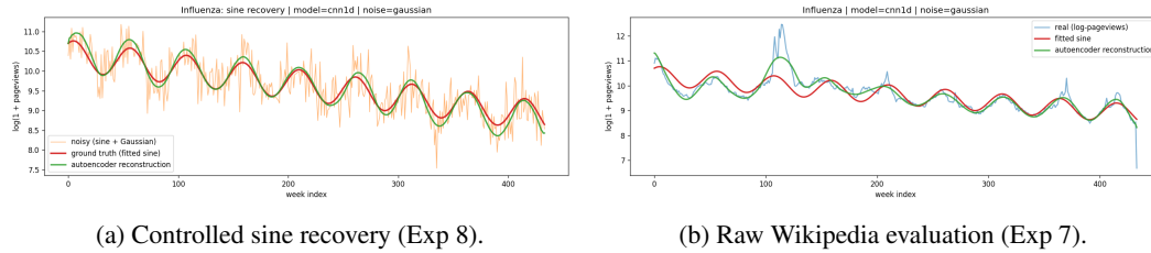
Figure 5: Two views of real-data behavior for Influenza. The left panel matches the synthetic task closely. The right panel shows the harder raw-series setting.
