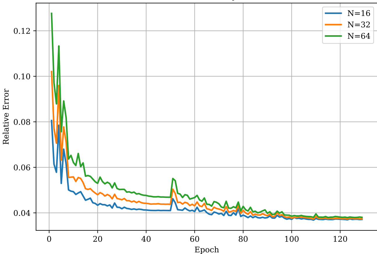
Validation Relative Error by Particle Count
