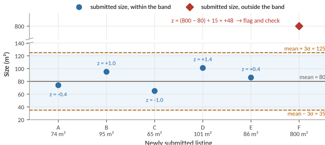
Figure 4.4 – The six submitted sizes against the training mean (80 m²) and the lines three standard deviations away (35 m² and 125 m²). The vertical axis is broken so that listing F fits on the page.
