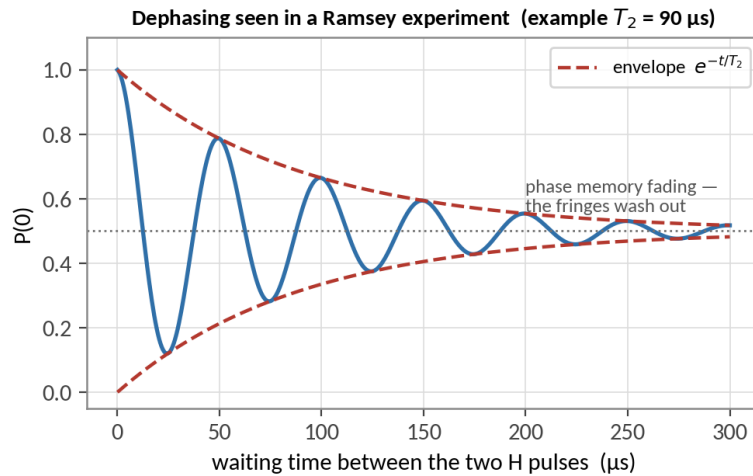
A Ramsey fringe decaying: the oscillation shows the accumulating phase; the shrinking envelope shows the phase becoming unreliable — superpositions aging into classical coin flips.
