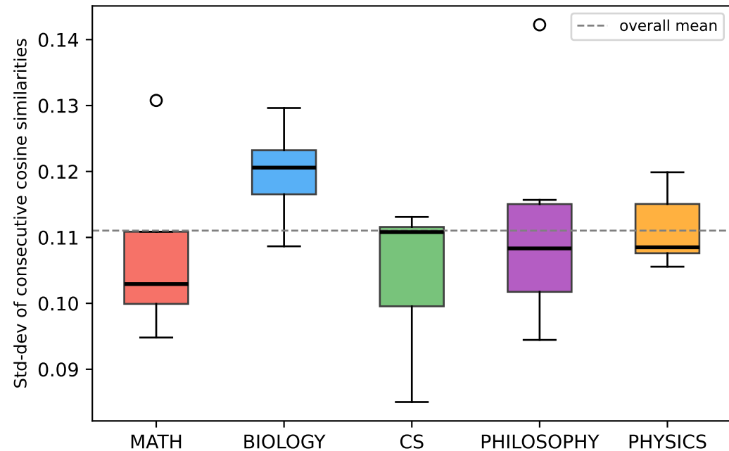
Embedding Variance Per Domain (higher = more discriminative boundary signal)
