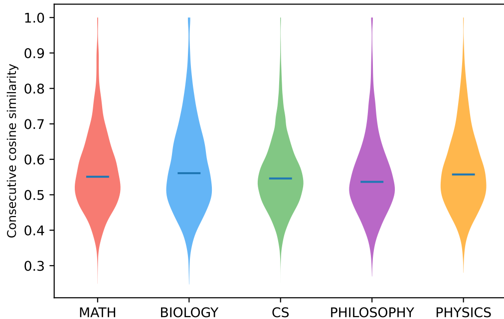
Distribution of Consecutive Similarities (MATH flat = low boundary discriminability)
