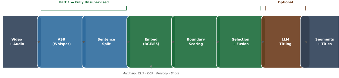
Figure 7.1: The LECSEG pipeline. Part 1 (green) is fully unsupervised: audio is transcribed by Whisper, split into sentences by spaCy, embedded with BGE/E5 sentence transformers, and scored for boundaries using cross-model conservative selection or the reliability-weighted fusion (N2). Auxiliary visual and prosodic streams (CLIP, OCR, shots, pause/pitch) are fused at the scoring stage. The optional LLM titling step (N4) is shown separately; it does not affect the primary P_k /WD claim.
