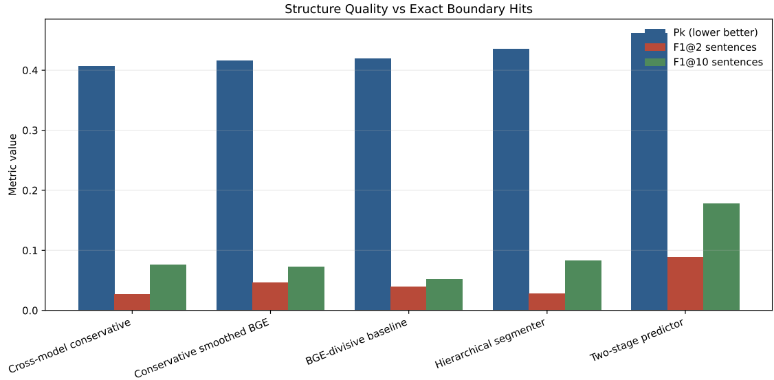
Figure 9.3: Diagnostic comparison between broad structure quality and strict boundary-hit metrics. Lower P_k is better; higher F1 is better. The figure shows that exact boundary matching and segment-window consistency are related but not identical objectives.
