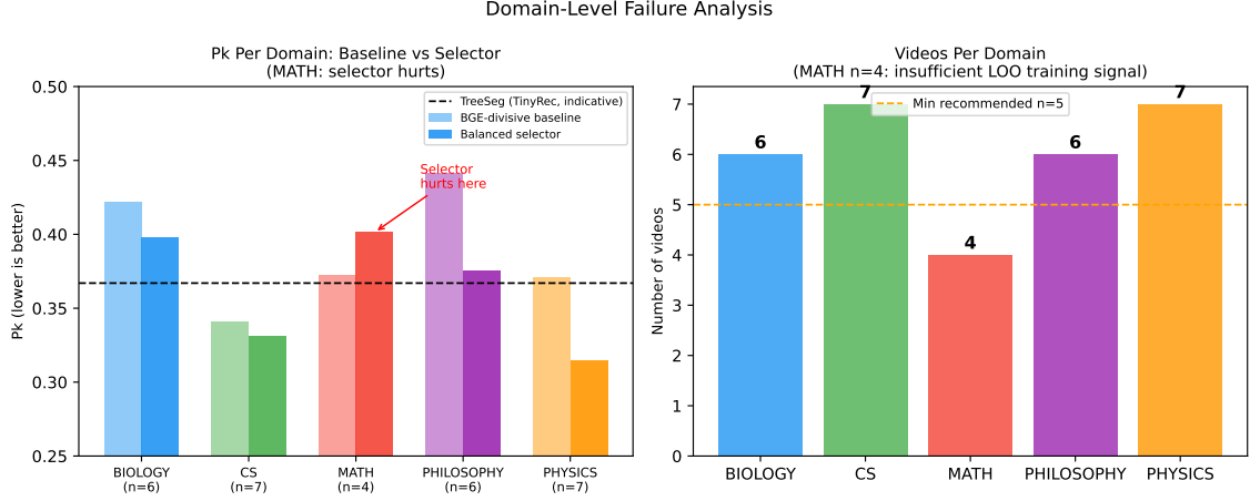
Figure 9.6: Domain failure analysis. Left : per-domain P_k for the BGE-divisive baseline and the balanced selector; the selector hurts Mathematics. Right : number of videos per domain. Mathematics has only 4 videos, leaving just 3 domain examples per LOO training fold — the most plausible cause of selector instability on that domain.
