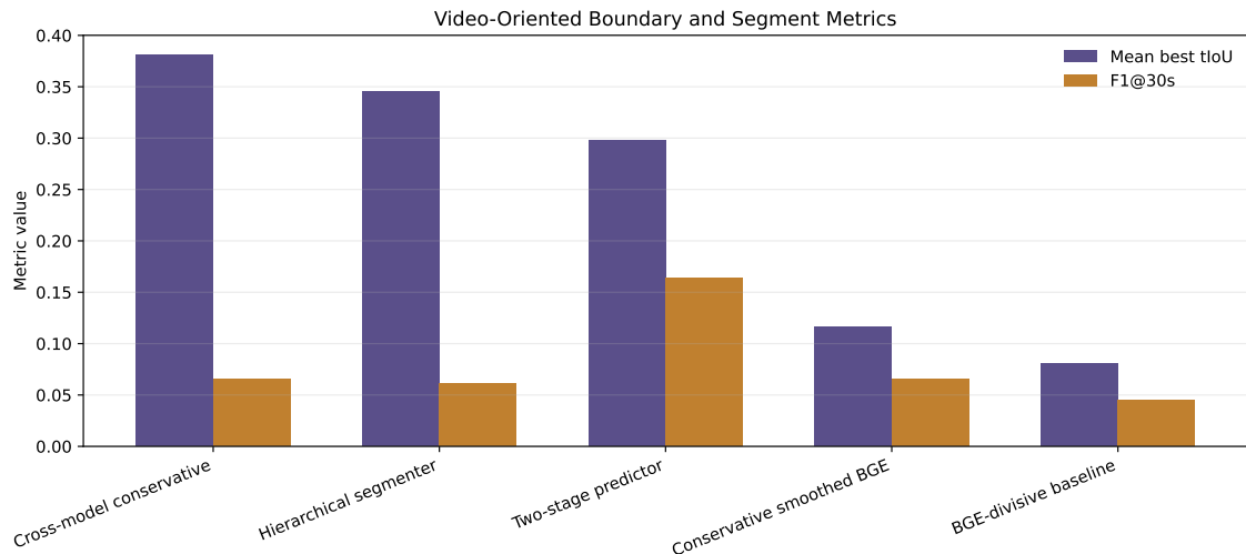
Figure 9.5: Video-oriented relaxed metrics: F1 within 30 seconds and mean best temporal segment overlap. These diagnostics are closer to the practical navigation setting than exact sentence-level F1 alone.
