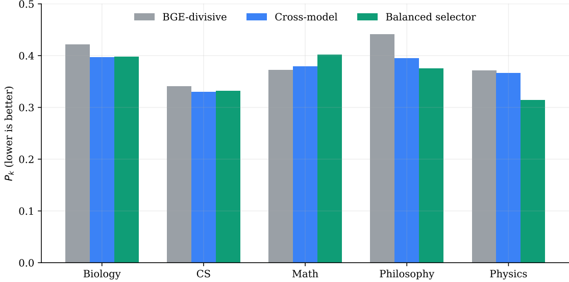
Figure 9.2: Domain-level P_k comparison. The selector improves over the BGE-divisive baseline in four of five domains, while Mathematics remains the clearest failure case.
