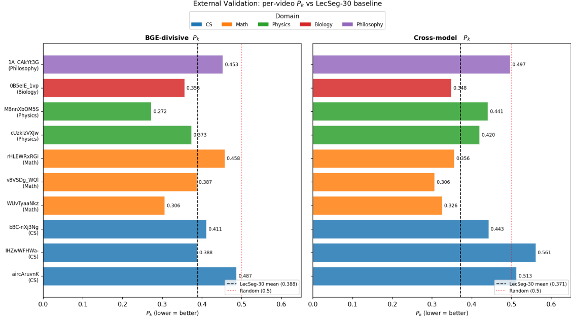
Figure 9.8: Per-video P_k on 10 external videos. Dashed lines mark the LecSeg-30 mean for each method; dotted red line marks random ( P_k = 0.5 ). Colour indicates domain.
