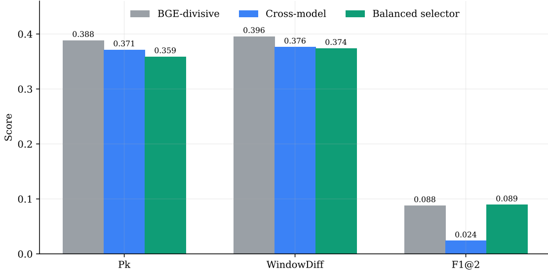
Figure 9.1: Primary LECSEG-30 operating points. Lower is better for P_k and WindowDiff; higher is better for F1@2. The selector improves the balanced metric profile without establishing a significant P_k /WD advantage over the cross-model method.
