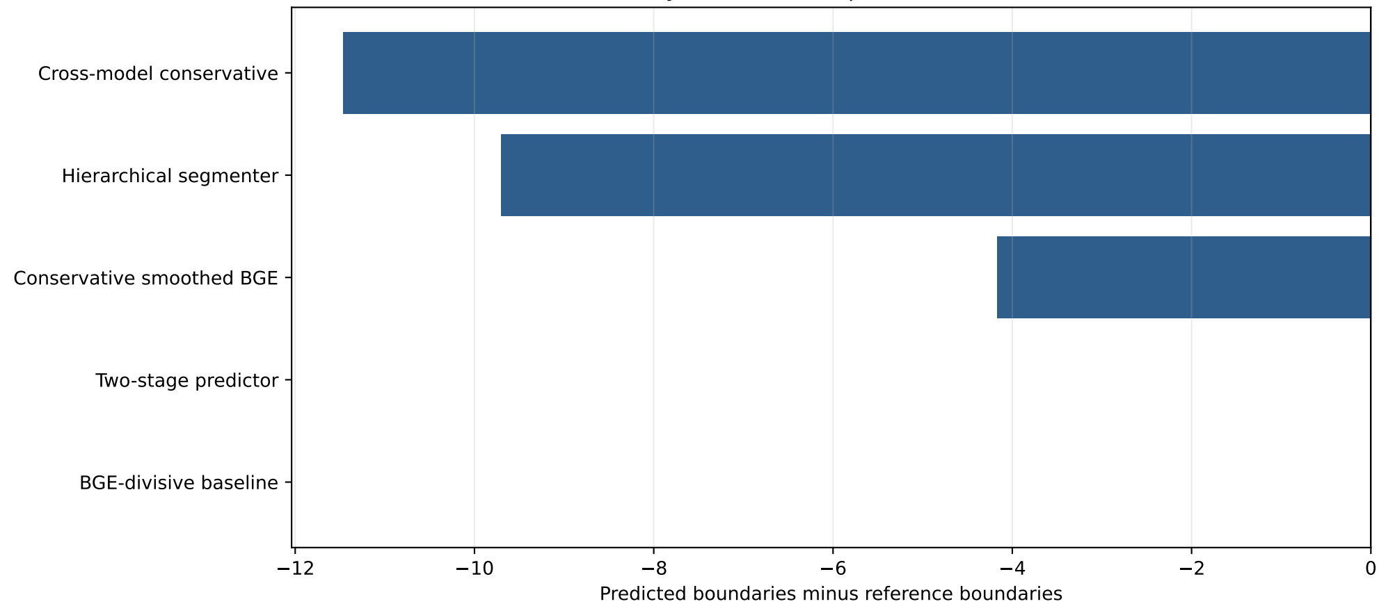
Boundary Count Error Explains F1/Pk Tradeoffs
