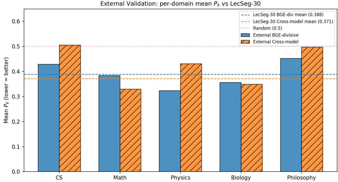
Figure 5.9: Per-domain mean P_k on external videos vs. LecSeg-30 means (dashed). Solid bars: BGE-divisive; hatched: cross-model.
