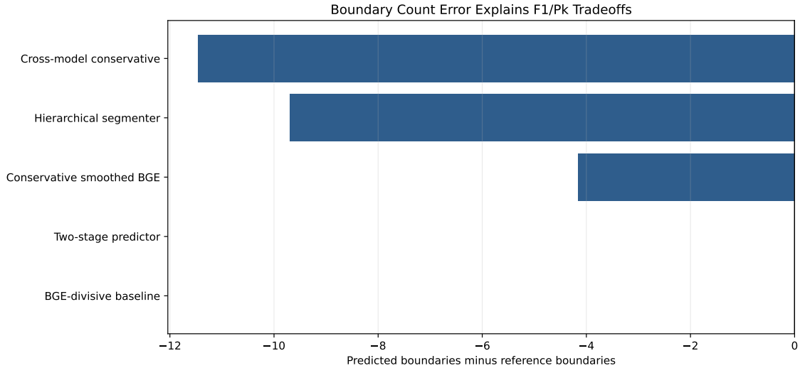
Figure 5.4: Mean boundary count error. Negative values mean a method predicts fewer boundaries than the creator reference; positive values mean over-segmentation. Count behavior explains why conservative methods can score well on P_k /WD while remaining weak on strict F1.
