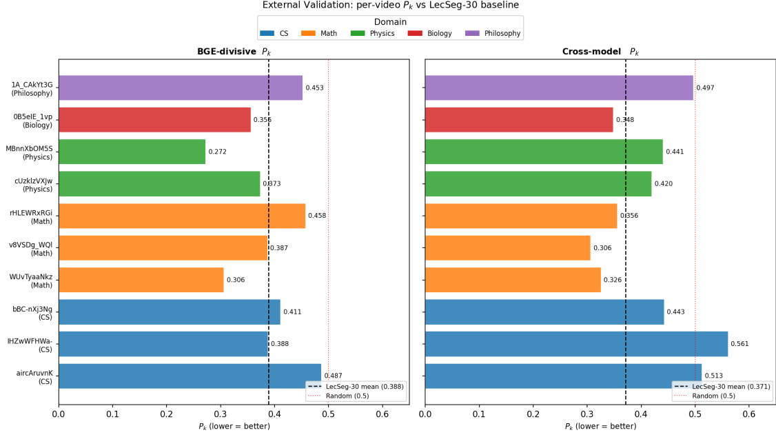
Figure 5.8: Per-video P_k on 10 external videos. Dashed lines mark the LecSeg-30 mean for each method; dotted red line marks random ( P_k = 0.5 ). Colour indicates domain.
