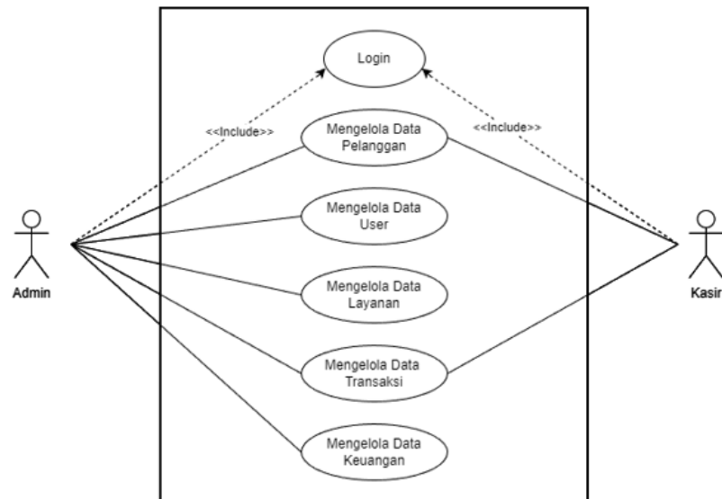
Gambar III.2: Usecase Diagram
