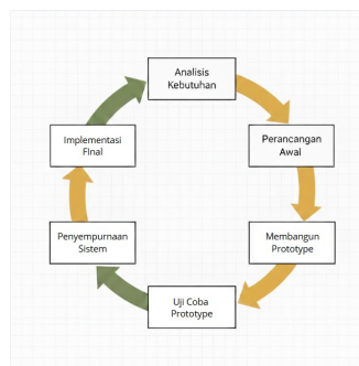
Gambar III.1: Prototyping
