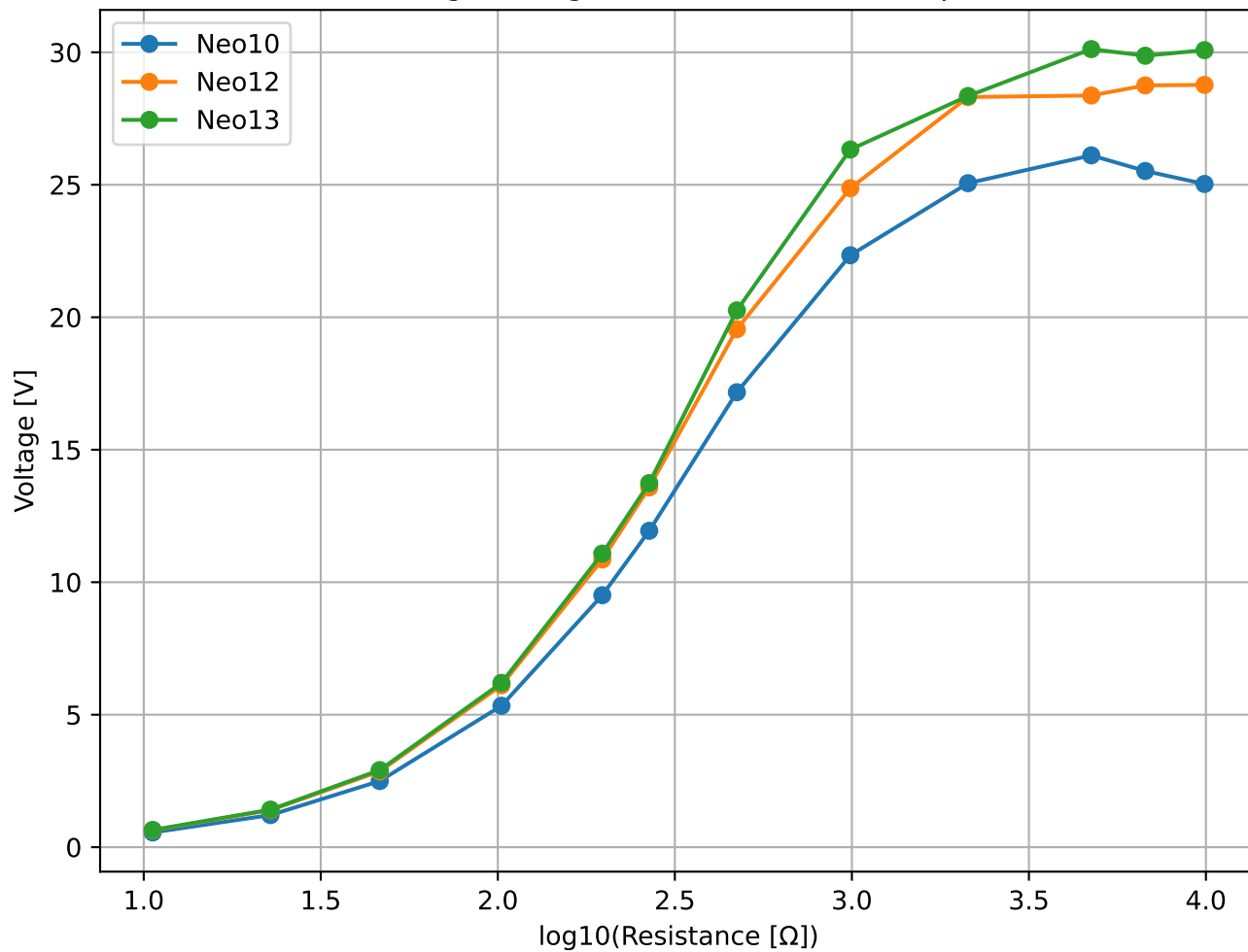
Voltage vs log10(Resistance) - 1260rpm
