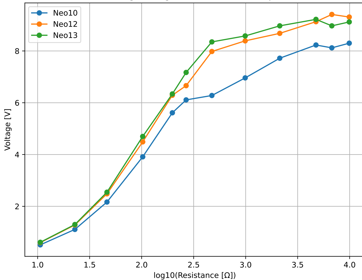
Voltage vs \log_{10}(\text{Resistance}) - 420rpm
