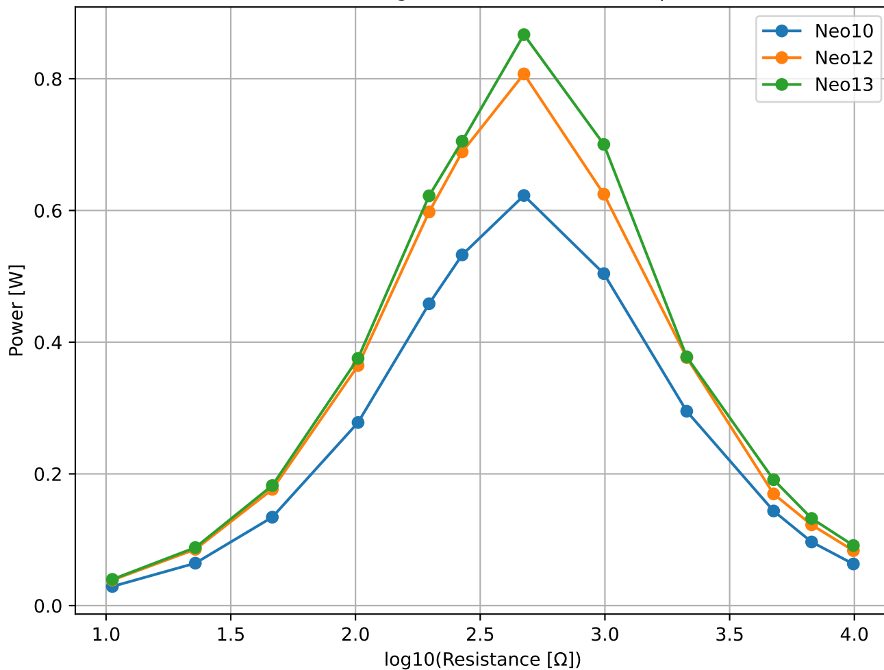
Power vs \log_{10}(\text{Resistance}) - 1260rpm
