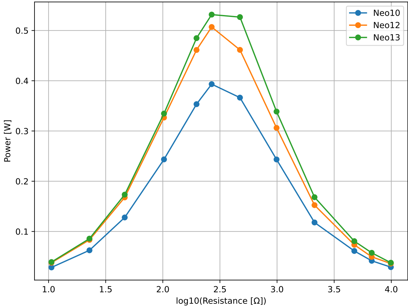
Power vs log10(Resistance) - 840rpm
