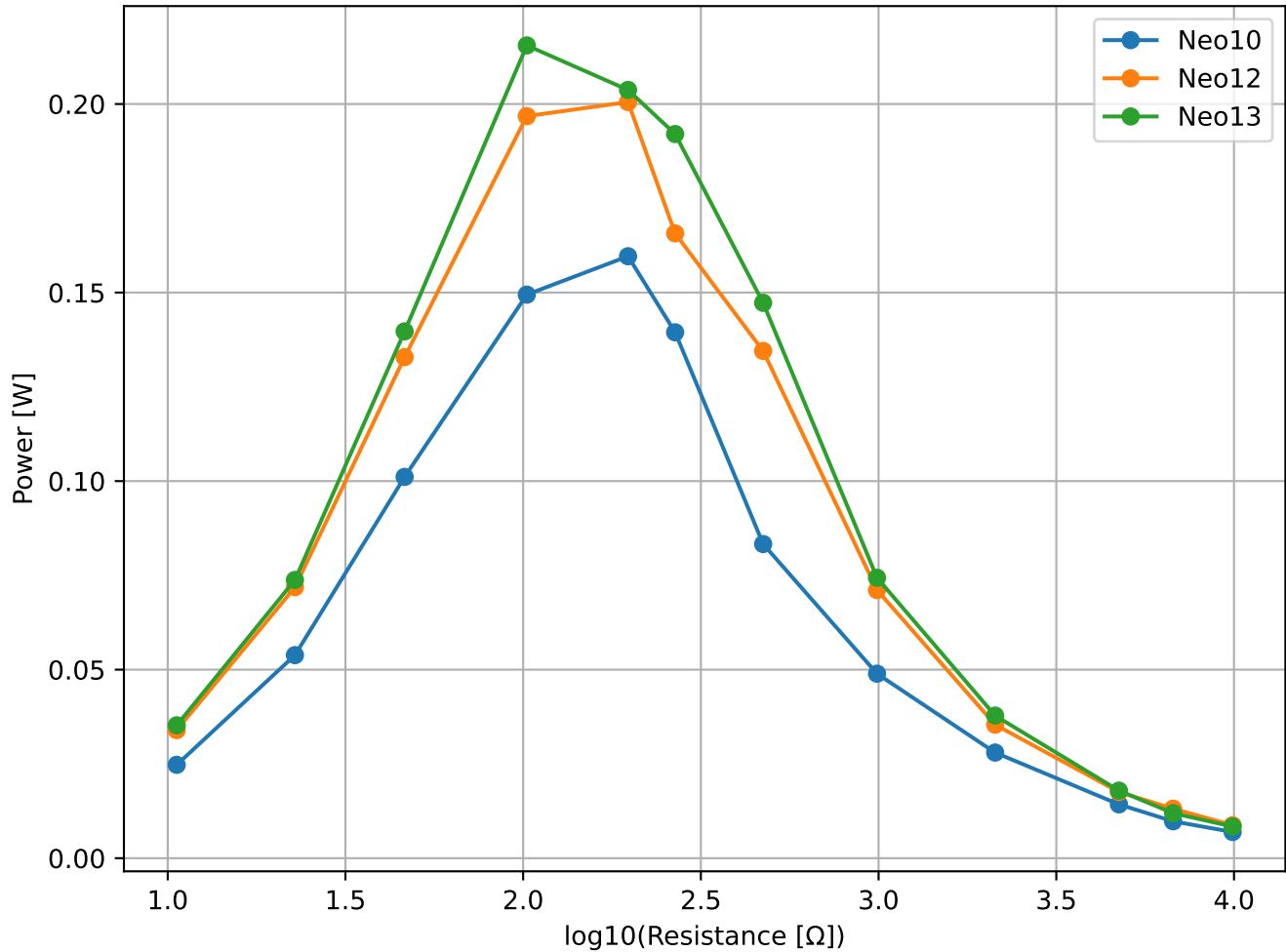
Power vs log10(Resistance) - 420rpm
